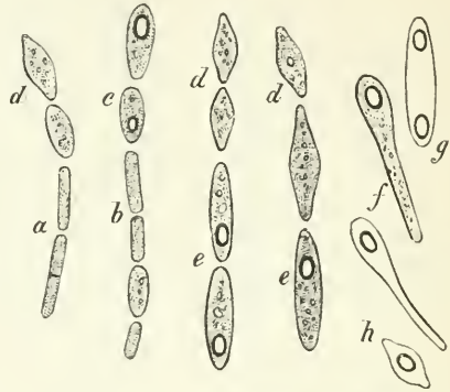
Fig. 12. Clostridium butyricum .
