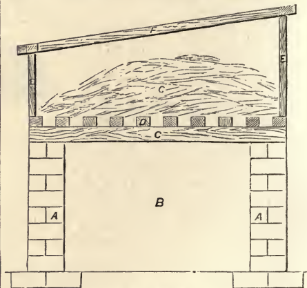
FIG. 563. SECTIONAL END VIEW OF A CHAMBERED FRAME.
