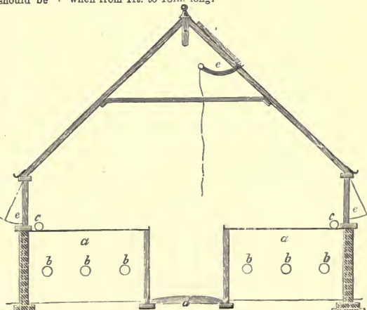
FIG. 560. SECTION OF SPAN-ROOF HOUSE.
