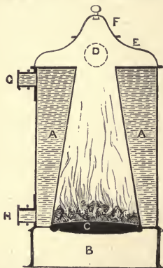
FIG. 260. VERTICAL SECTION OF CYLINDER BOILER.
