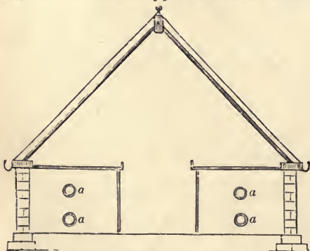
FIG. 562. SECTION OF SPAN-ROOF HOUSE.
