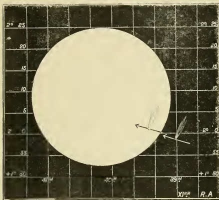
Ingress of Gould's Comet upon Sun, September 17, 1882.
