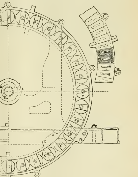
FIG. 6.—Elevation of Gordon's Dynamo, showing the rotating coils. The "taking-off" coils are shown in the top right hand corner.
