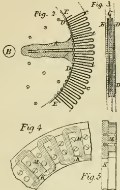
FIGS. 2-5.—Sir W. Thomson's Disk-Dynamo
