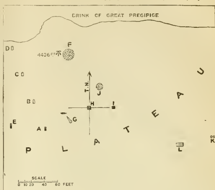
FIG. 3.—A, B, C, D, rain-gauges; E, notice board; F, Ordnance Survey cairn; G, solar and terrestrial radiation thermometers; H, Stevenson's thermometer cage and ozone tests; I, self-registering hygrometer; J, barometer cairn; K, earth thermometers; L, hut. The apparatus for measuring the actinism of light is near the edge of the precipice N.E. from the hut.
