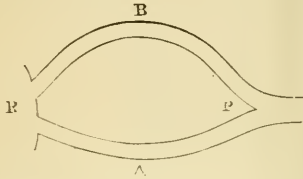
FIG. 2.—Diagram to illustrate Sir J. Herschel's observations on interference. Adapted from his article on "Absorption of Light," Phil. Mag. 1863, p. 405.
