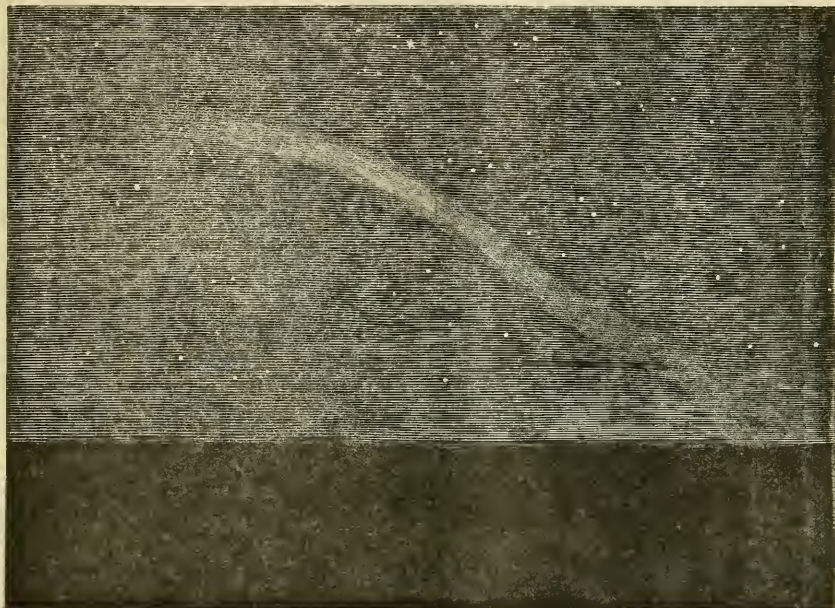
Auroral Arch, observed November 2, 1871, at Groningen (Netherlands).
