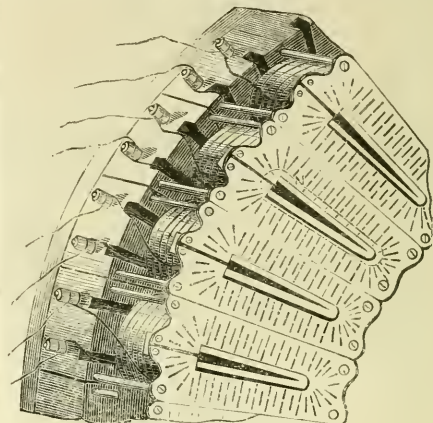
FIG. 8.—The Fixed Coils of Gordon's Dynamo.
