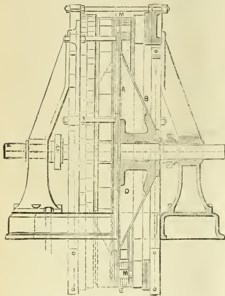
FIG. 7.—End Elevation and Section of Gordon's Dynamo.
