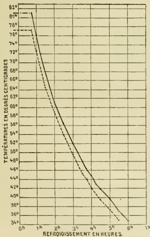
FIG. 2.—Curves of cooling of warming-pans with water.
