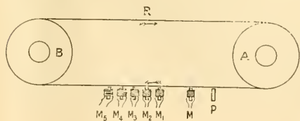
FIG. 3.—Distributing Telegraphone.
