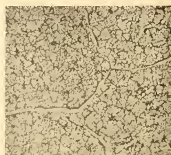
FIG. 3.—Chilled at 500°.
