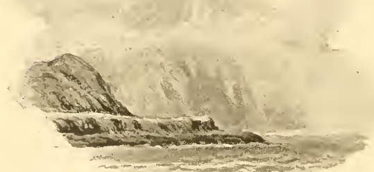
FIG. 3.—Rock terraces of old sea margins, Isle of Jura.
