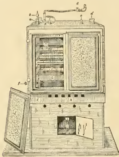
2296. Standard seed-germinating chamber (front view, with one door slide removed).
