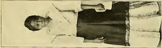
FIG. 4. PRIMITIVE (BLEND).
