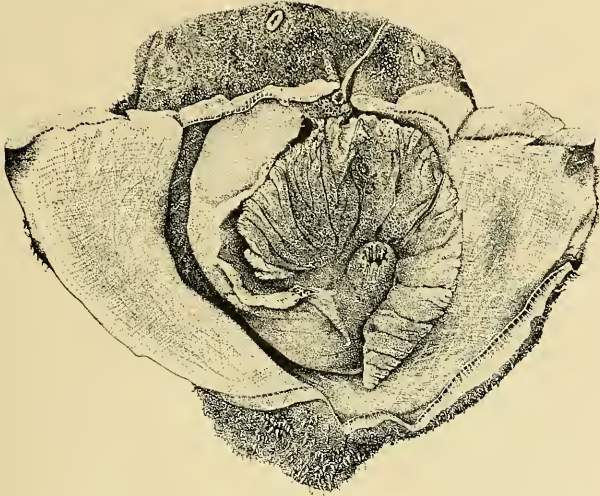
Fig. 8. Branchial cavity of aclesia.
