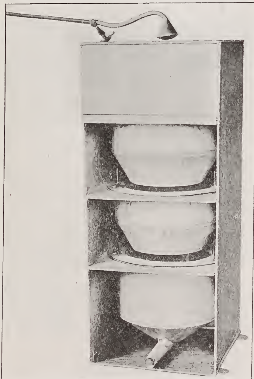
Fig. 1. Apparatus for obtaining insects, etc., from soil ; \times \frac{1}{10} .
