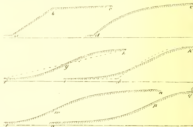
Fig. 51.—Good and Bad Slopes.
