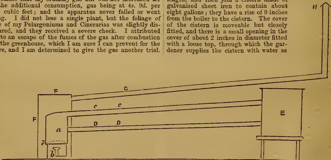
a, Boiler. b, Bunsen's burner.
