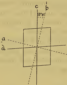
Fig. 4. Schizolite, optic scheme.
