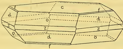
Fig 6. Steenstrupite, type II.
