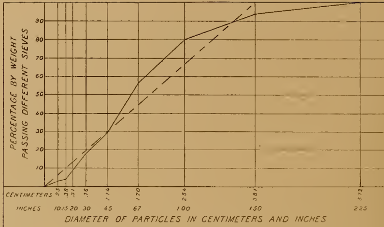
FIG. 14.—GRANULARMETRIC ANALYSIS OF MARIQUINA GRAVEL TO PASS A 1.5-INCH OPENING.
