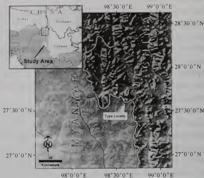
Fig. 10 Map of the Gongshan study area(insert: study area outlined in white; black box locates area of enlargement) Sites at which specimens of Aristochroa abrupta sp. nov. were collected are identified by solid white circles and the type locality by a star
