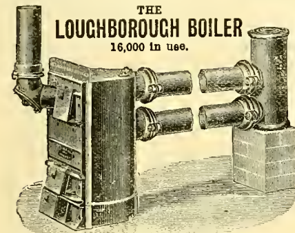
The Pioneer of cheap, simple, and effective heating for small Greenhouses.
