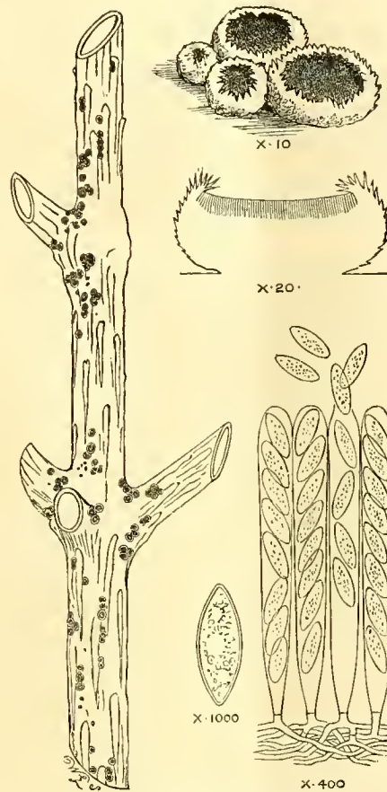
FIG. 65.—PEZIZA WILLKOMMII: Cluster Cups magn. 10 diam.; Section of Cup magn. 20 diam.; Spore Capsules or Asci magn. 400; separate Sporidium, magn. 1000.
