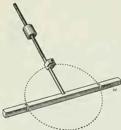
FIG. 5.—Diagram showing the construction of knife-edges. The square rod is milled halfway through at points where it engages the walls of the pot in order to reinforce the cement joint.
