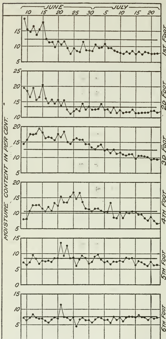
FIG. 8.—Chart showing the daily moisture determinations in 1-foot sections to a depth of 6 feet in a soil on which Kubanka wheat was growing. The heavy horizontal straight lines on the chart represent the wilting coefficient as calculated from the moisture equivalent independently of the moisture determinations or of field observations. The wheat wilted on July 1 and was cut July 22. The graphs show that the moisture curves are either coincident with or below the wilting coefficient on July 1, indicating that there was no longer moisture available for growth. The continuous loss of water from the soil after wilting takes place is also shown.
