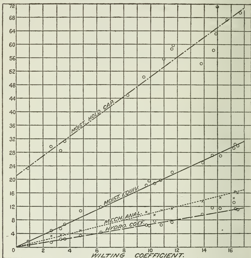
FIG. 9.—Chart showing the linear relationship between the wilting coefficient and physical measurements of the moisture retentiveness of soils. The wilting coefficient is represented by the axis of abscissas, while the axis of ordinates for the different graphs represents the moisture retentivity of the soil as measured by the hygroscopic coefficient, the moisture equivalent, and the moisture-holding capacity, and as computed from the mechanical analysis. The quantity employed as ordinate in each case is designated on the graph.
