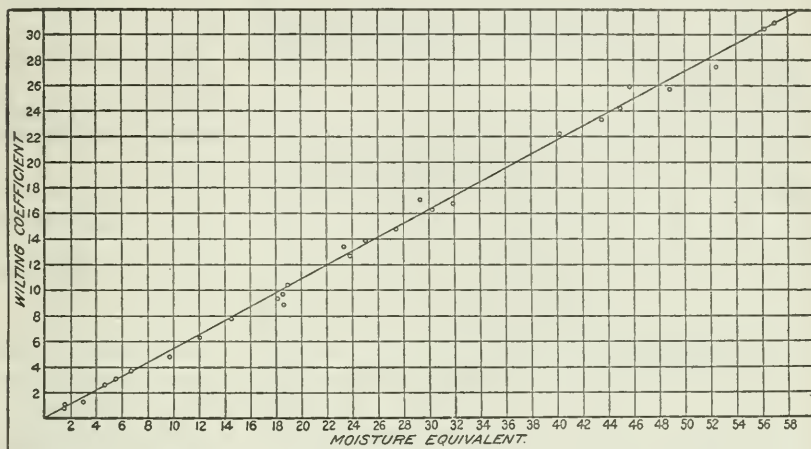
FIG. 7.—Chart showing the linear relationship between the wilting coefficient and the moisture equivalent for 28 types of soil ranging in texture from coarse sands to the heaviest clays.
