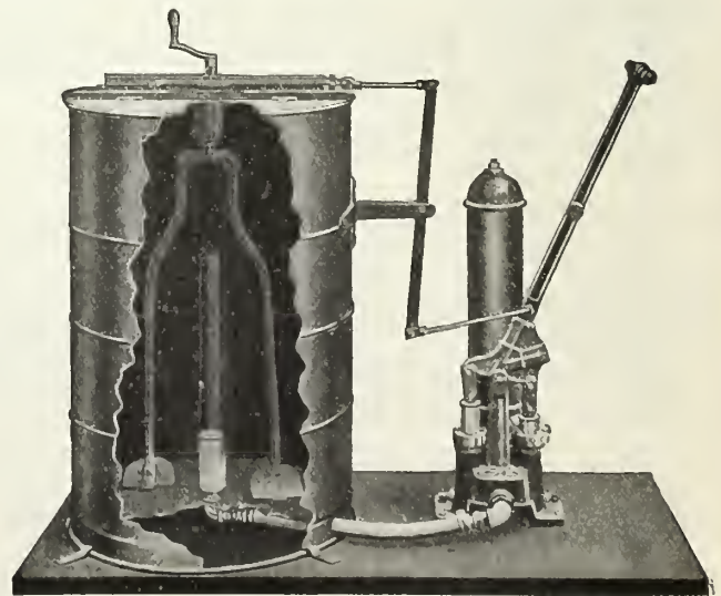
Cobb Park and Farm Sprayer.
