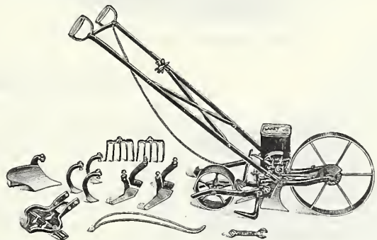
Planet Jr. No. 28. Combined Hill and Drill Seeder, Wheel Hoe Cultivator, Rake and Plow.
