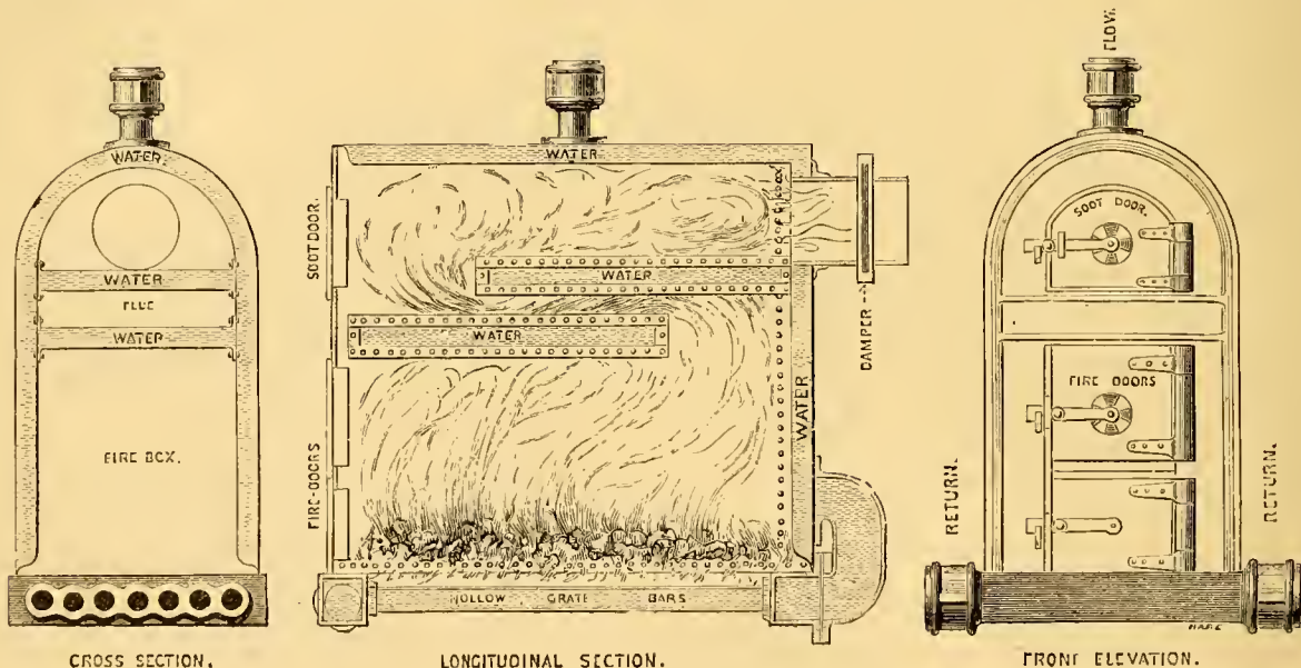
Green's Patent Wrought-iron Boiler.
