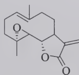
parthenolide
