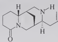
angustifoline
