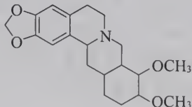
berberine
