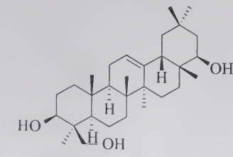
soyasapogenol A
