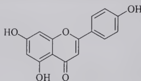
apigenin
