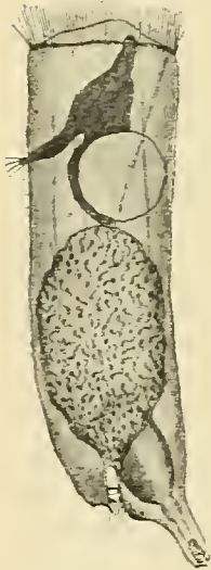
Megalotrocha alboflavicans Ehrbg. ♂ after Hlava.
