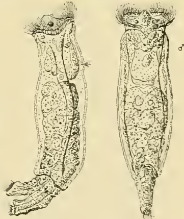
Pterodina elliptica ♂ after Rousselet.
