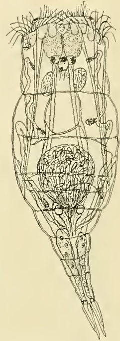
Eosphora digitata ♂. Ehrbg. after de Beauchamp.
