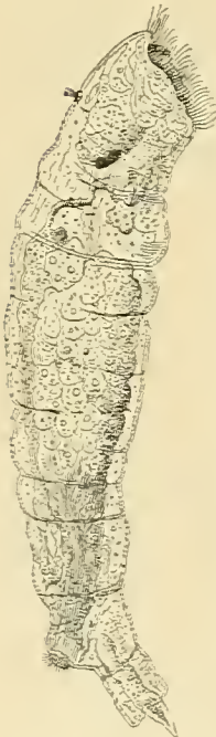
Proales Wernecki ♂ Ehrbg. after Rousselet.
