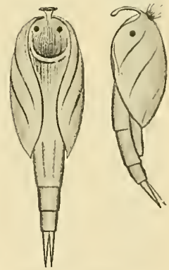
Colurus bicuspidatus ♂ after Weber.
