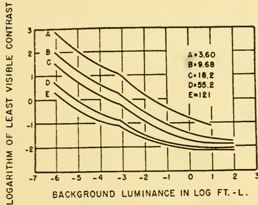
Fig. 34. Visibility of objects as a function of background luminance and size of object. The object sizes, A, B, C, D, and E, are in minutes of visual angle. (After Blackwell, 2)
