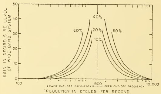
Fig. 2. Equal-articulation contours for band-pass systems in noise. The parameter is the articulation score. The abscissa indicates the lower and upper cut-off frequencies of the band. The ordinate gives the increased amplification necessary for the narrow-band system to maintain the same articulation score as a wide-band system. Men's voices. (After Egan and Wiener, 9)
