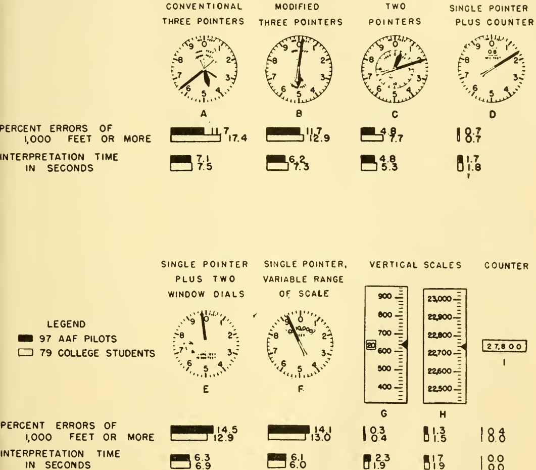
Fig. 11. Reading altitude from different types of instruments. Data from Grether (31) for 176 subjects, each of whom made 12 readings on each type of instrument. The results given below each illustration show the percentage of readings which were in error by 1000 feet or more and the instrument interpretation time in seconds. The latter was assumed to be zero for the counter, so counter-test time, essentially number-writing time, was subtracted from all other instrument test times to obtain their interpretation times.
