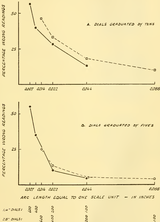
Fig. 7. Frequency of reading errors for dials graduated by tens and by fives. Data from Kappauf and Smith (41) for six subjects, each of whom made 30 readings for each type and size of dial under instructions to be as accurate as possible. Brightness level: six foot lamberts.
