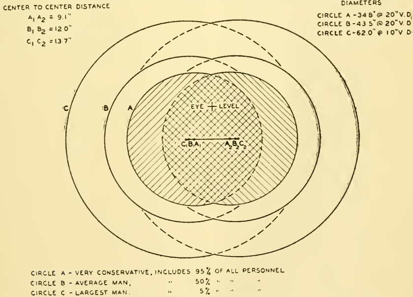
Fig. 5. The limits of maximum working areas on a vertical surface. (After Lipschultz and Sandburg, 24)
