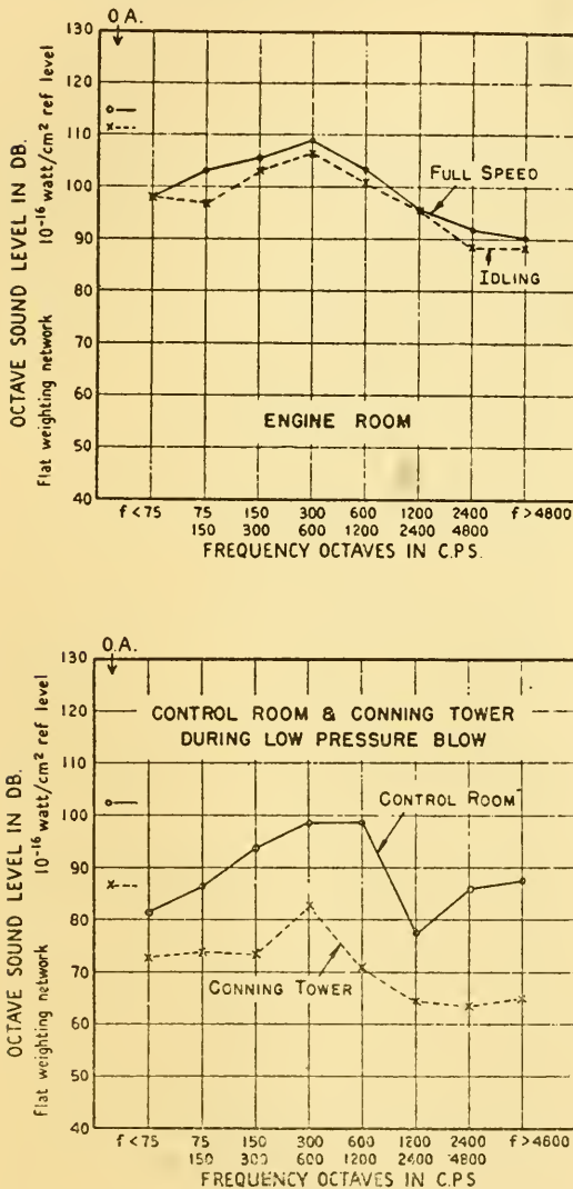
Fig. 1. Examples of noise spectra found in USS REDFISH. The symbol O.A. refers to overall sound pressure level. The sound pressure levels measured in successive bands one octave wide are shown by the points on the curves.
