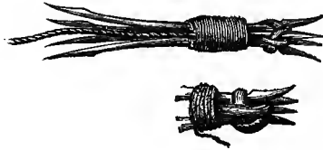
CAYMAN HOOK.
