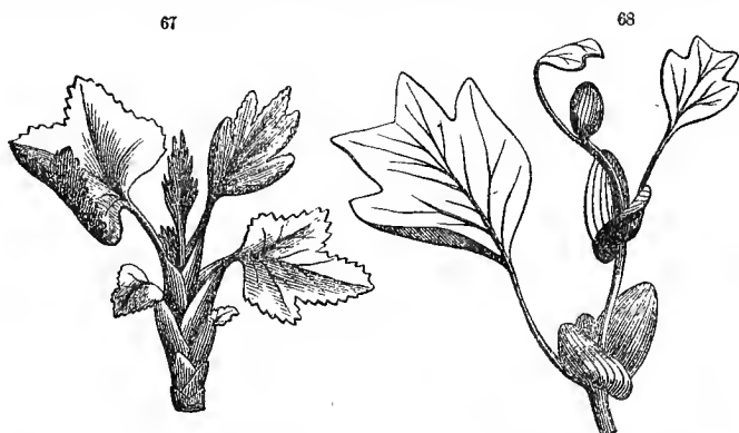
67, Bud of currant unfolding,—the scales gradually becoming leaves. 68, Bud of tulip-tree,—the scales unfolding into stipules.
