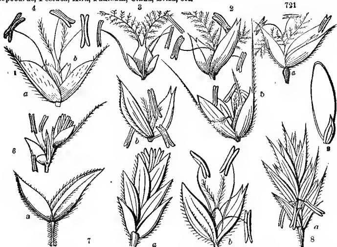
FIG. 721. Agrostis alba ; a 1-flowered spikelet; a, the two glumes. 2. A flower, with the two paleæ, three stamens and two plumous stigmas. 3. Leersia oryzoides ; a flower removed from its glumes, showing its 2 hypogynous scales, three stamens and ovary with the two stigmas. 4. Phleum pratense ; a 1-flowered spikelet; a, glumes; b, truncate paleæ; etc. 5. Polypogon ; a 1-flowered spikelet; glumes and lower paleæ awned. 6. Holcus lanatus ; a 2-flowered spikelet; a, glumes; b, the two flowers (upper staminate). 7. Poa pratensis ; a 4-flowered spikelet; a, the two glumes; b, a single flower, with two paleæ, etc. 8. Festuca duriuscula ; a 5-flowered spikelet; a, two glumes; b, a single flower. 9. The caryopsis of Hordeum , showing the embryo at the base of the copious albumen.
