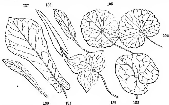
Forms of leaves. 130, Silene Virginica .. 131, Magnolia Fraseri . 136, Arabis dentata . 137, Polygonum arifolium . 132, Hepatica acutiloba . 133, Asarum Virginicum . 134, Hydrocotyle Americana . 135, H. umbellata .
