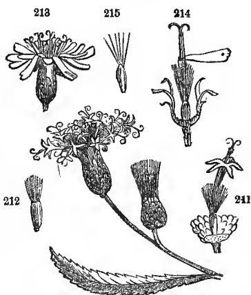
Vernonia fasciculata ; flowers in a discoid head with an imbricated involucre. 211, A single flower remaining on the receptacle. 212, A fruit crowned with the pappus. 213, Mulgodium; a head. 214, A single flower remaining on the receptacle. 215, A fruit with pappus.
