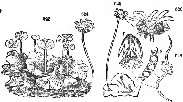
Hepaticæ. 523, Marchantia , sterile plant. 524—5, Fertile plant. 526, Vertical section of the fertil-receptacle; 527, of a perianth, showing the sporangium bursting. 528, One of the elators with four spores. 529, Portion of it highly magnified.
