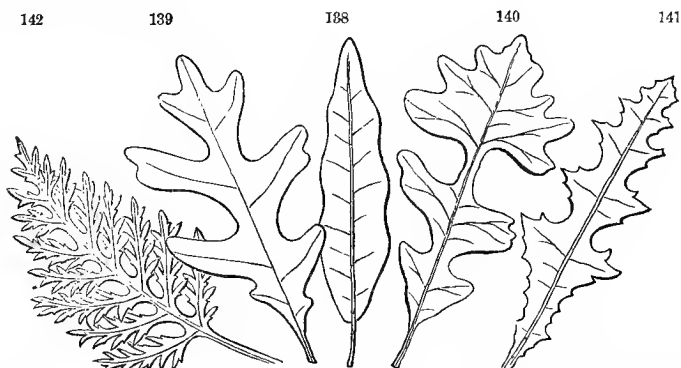
Feather-veined leaves, approaching the compound. 138, Quercus imbricaria —undulate. 139, Q. alba (white oak)—lobate-sinnate. 140, Q. macrocarpa —lyrate. 141, Mulgedium (milk-weed). 142, Bipinnatifid leaf of Ambrosia artemisifolia (hog-weed).
