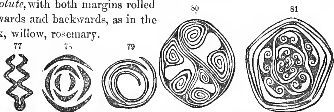
Vernation. 77, of birch leaf; 78, of lilac, (imbricate); 79, cherry leaves, (convolute); 80, dock bud, (revolute); 81, bala of Gilead, (involute).
