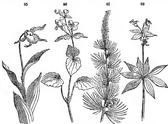
85, Ladies'-slipper (leaves alternate); 86, Synandra grandiflora (leaves opposite); 88, Medeola Virginica (leaves verticillate); 87, Larix Americana (leaves fasciculate).
