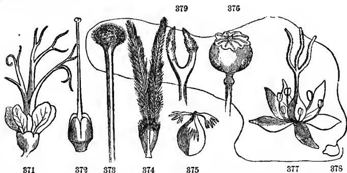
Pistils. 372, Symphytum , basilar style, ovary 4-parted. 371, ♀ Fl. of Emblica ( Euphorbiaceæ ), branching styles. 373, Mirabilis Jalapa , globular stig. 377, Fl. of Luzula , stigmas linear. 374, Feathery stigmas of a grass. 379, Stigmas of Aster . 375, Rumex . 376, Poppy. 378, Filiform stigma of Zea Mays , (Corn).
