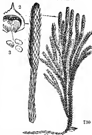
730, Lycopodium dendroideum . 731, A single spike. 732, A scale with its axillary sporangium bursting. 733, Spores.
