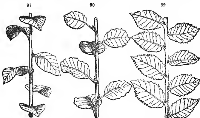
Phyllotaxy. 89, leafy branch of elm,—cycle \frac{1}{2} . 90, leafy branch of alder,—cycle \frac{1}{3} ; 91, leafy branch of cherry,—cycle \frac{2}{5} .
