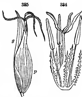
334, Flower of Scirpus lacustris , magnified; consisting of six setae, three stamens, three pistils united, except the stigmas. 335, Flower of Carex rivularis ♀, with g , its glume, p , its bottle-shaped perigynium, 2-toothed at top, enveloping the triple ovary; stigmas, three.
