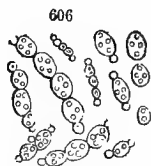
606, Penicillium glaucum , the Yeast-plant.
