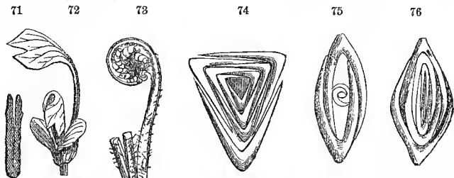
Vernation, 71, of oak leaf; 72, of Liriodendron (tulip tree); 73, of fern; 74, of carex ; 75, sago; 76, iris.
