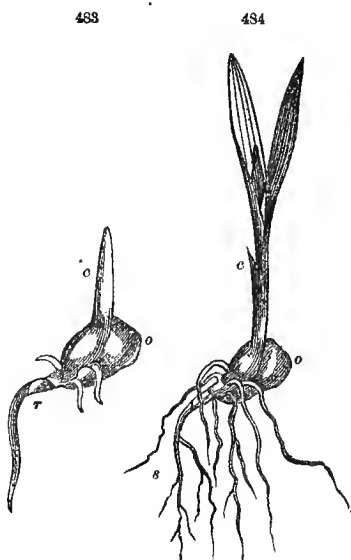
483, 484, Germination of Indian Corn.
