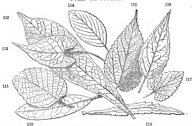
Forms of leaves. 110, Rhododendron maximum . 111, Alnus glutinosa (cult.). 112, Polygonum sagittatum . 113, Pawpaw. 114, Impatiens fulva . 115, Celtis Americana . 116, Cirenea Lutohana . 117, Catmint. 118, Solidago Canadensis —a triple-veined leaf.
