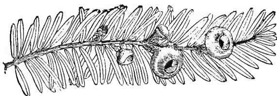
FIG. 692. Taxus Canadensis —naked seeds.
