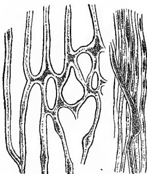
Vessels of Cienchyma; 530, from Dandelion; 531, from the Celandine.
