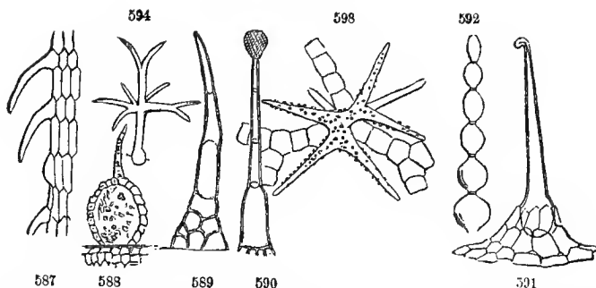
587, Rootlet of Madler, showing cells expanded into fibrillae. 588, Glandular hair of Ficus , section. 589, Hair of Bryonia , of several cells. 590, Hair of several cells, surmounted by a gland, of Antirrhinum majus . 591, Sting of Urtica dioica . 592, Jointed hair of the stamens of Tradescantia . 593, Stellate hair from the petiole of Nuphar advena (magnified 200 diameters, Menfey). 594, Branched hair, one cell, of Arabis .
