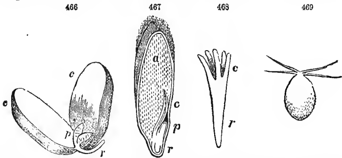
466, Dicotyledonous (Bean). 467, Monocotyledonous (Wheat). 468, Polycotyledonous (Pine). 469, Acotyledonous (zoospore of one of the Conservæ). ( r , r , r , radicle; p , p , p , plumule; c , c , c , cotyledon; a , albumen).
