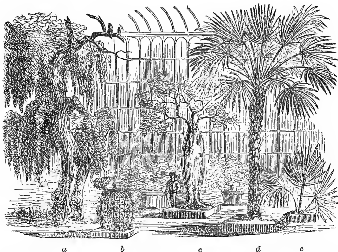
47. a , An old willow ( Salix Babylonica ) with gnarled and misshapen trunk. b , Caudex of a cactus ( Echinocactus Ottonis ). c , Bombax , of Brazilian forests, with distended trunk. d , Palmetto ( Sabal , Adns ), the caudex rough with the persistent bases of the petioles.
