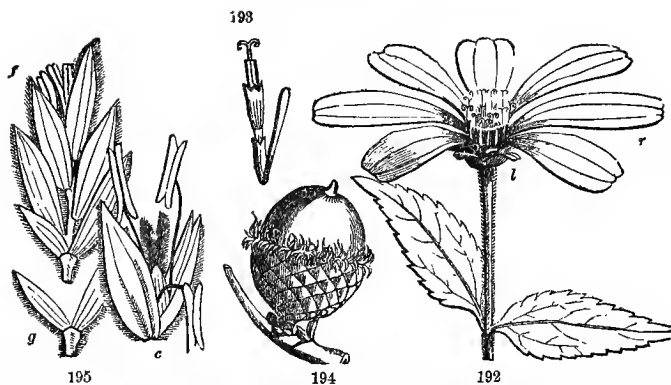
192, Helianthus grosse-serratus . l , involucre; r , rays, or ligulate flowers; 193, one of the disk flowers with its chaff-seal (bract). 194, Acorn of moss-cup oak ( Q. macrophylla ). 195, Poa pratensis ; f , spikelet entire, g , glumes, separated; c , a flower separated, displaying the two paleæ, 3 stamens, and 2 styles.
