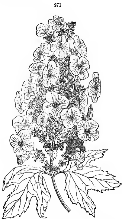
271, "Radiant" panicle of Hydrangea quercifolia ; the larger flowers neutral.
