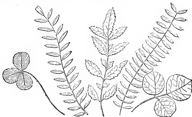
157 161 159 160 158 Compound leaves. 157, Trifolium repens . 158, Desmodium rotundifolium . 160, Glutidium . 161, Cassia . 159, Agrimonia .
