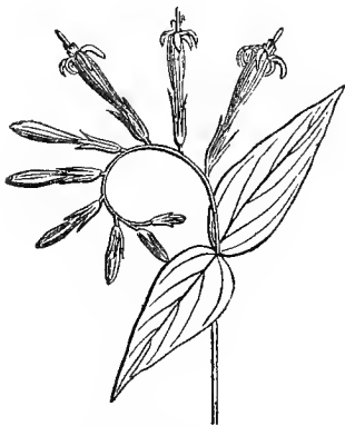
221, Spigelia Marilandica ; a scorpoid raceme.
