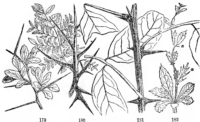
Thorns. 179, Crataegus parvifolia (thorns axillary.) 180, Honey-locust. 181, Common locust. 182, Berberis , \alpha , \alpha , its thorns.
