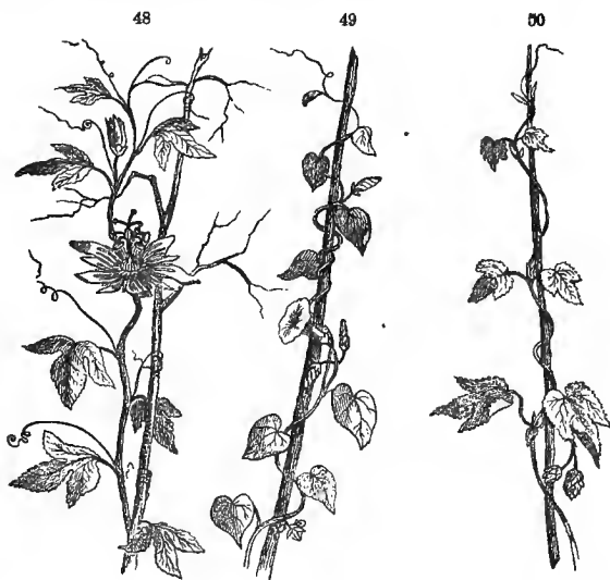
Vines. 48, Passion-flower ( Passiflora lutea ) climbing by tendrils. 49, Morning-glory, twining from right to left. 50, Hop, twining from left to right.
