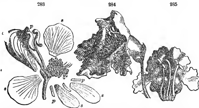
283, Flower of Aconitum Napellus displayed; s, s, s, s, s , the five sepals, the upper one hooded; p, p, p , the five petals, of which the two upper are nectaries covered by the hood, and the three lower very minute. 284, Flower of Catalpa , 2-lipped, 5-lobed. 285, Corolla laid open, showing the two perfect etamens and the three rudimentary.
