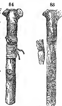
83, 84, Showing the process of "budding."
