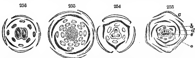
Diagrams of flowers (as seen by cross-sections). 253, Jeffersonia diphylla : o , ovary; s , stamens; d , inner row of petals, æstivation triquetrous; h , outer row of petals, æstivation contorted; c , sepals, æstivation quincential. 254, Lily. 255, Strawberry. 256, Mustard. The pupil will designate the modes of æstivation.
