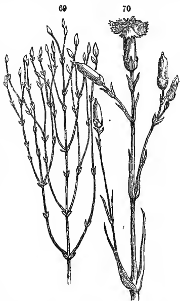
69, Hypericum Sarrothra , with brachiate branches. 70, Pink ( Dianthus )—axillary buds alternately suppressed.
