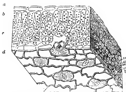
604, Minute portion of a leaf of Viola tricolor , viewed in perspective, showing, a , cells of epidermis above; b , compact parenchyma of the upper portion of the leaf; c , loose parenchyma; d , epidermal-cells of the lower surface with stomata, one cut and opening into the intercellular passages. (Magnified 100 diameters.)
