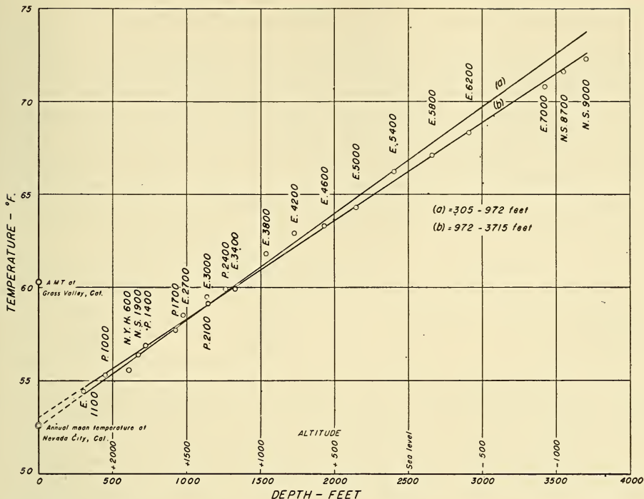
Fig. 1.—Depth-temperature relation, Empire-Star Mine, Grass Valley, Calif.
