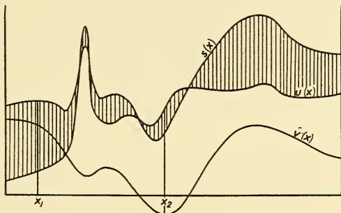
Fig. 5.—Graphical addition of vectors in function space.
