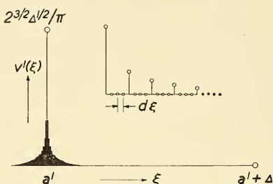
Fig. 3.—The same vector \mathbf{v} (Fig. 2) represented in terms of a new coordinate system \mathbf{e}_\alpha^0, \mathbf{e}_\beta^0, \dots, \mathbf{e}_\nu^0 . In the inset the \xi -axis has been infinitely magnified to show the details close to the point \xi = a' . The actual width of the shaded block at a' is infinitesimal.
