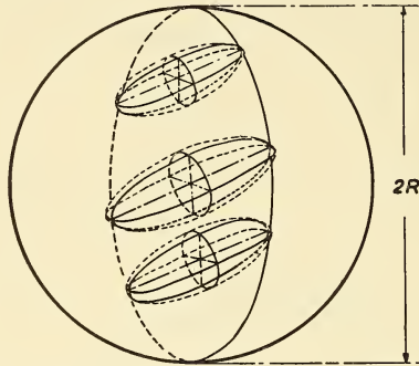
Fig. 4.—Projected sections of a hypersphere.
