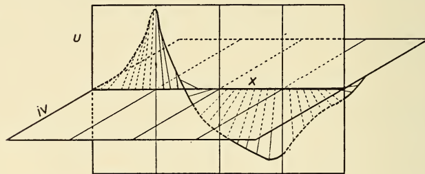
Fig. 2.—An n -component bi-vector in function space.
