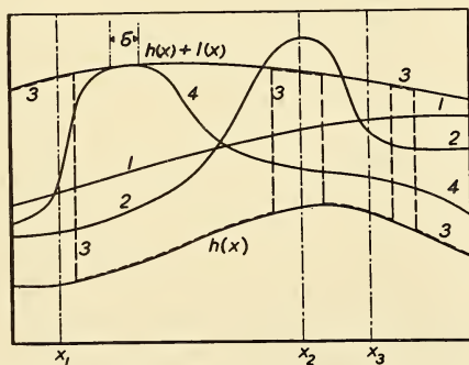
Fig. 9.—Function space diagram of a rectangular hyperparallelopiped.
