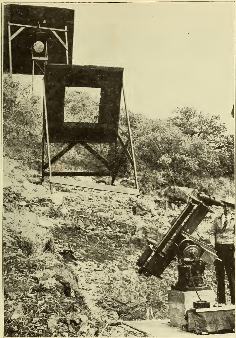
Fig. 4.—Nebular spectrograph of the McDonald Observatory.
