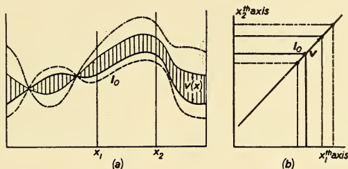
Fig. 7.—(a) Representation of a line in function space; (b) its principal projection on the x_1, x_2 plane.
