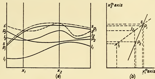
Fig. 9.—Construction for locating intersection of two straight lines in function space.
