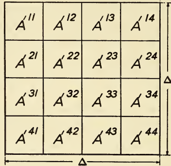
Fig. 5.—Matrix of 2-rank and 4-order.
