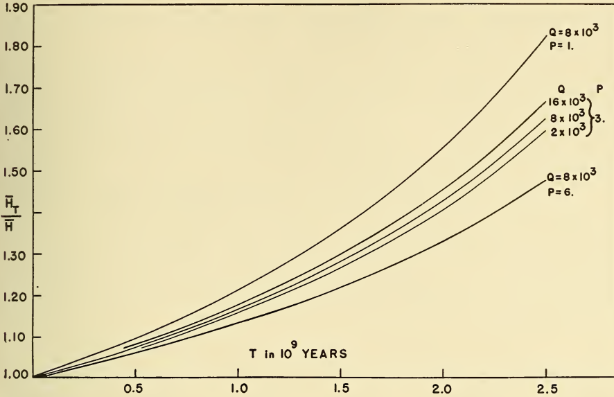
Fig. 3.—The ratio of the rate of production of heat, from all the known radioactive sources, in the past to the value at present, (\bar{H}_T/\bar{H}) , as a function of time T in the past.
