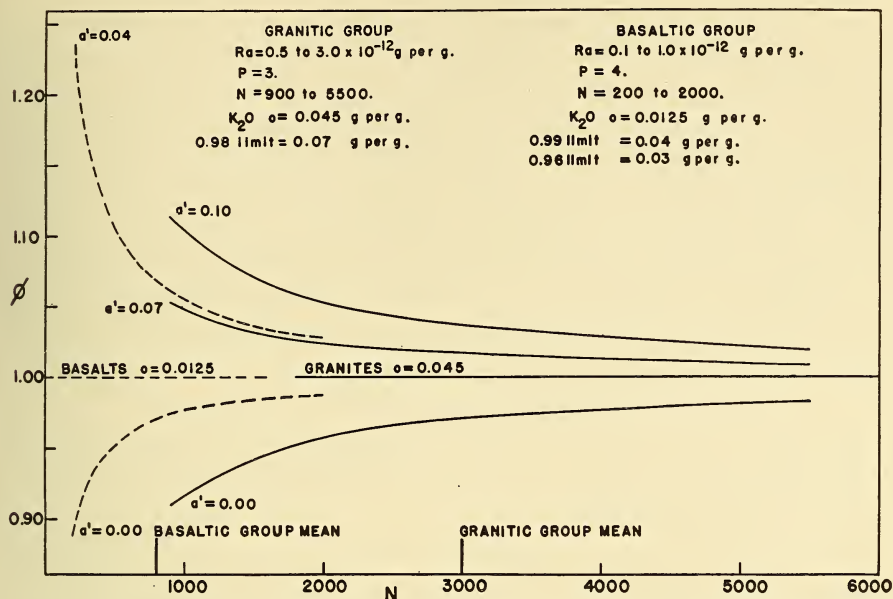
Fig. 1.—The uncertainty ratio \phi as a function of the alpha-particles emitted per hour, N , for the granitic group as defined in the text, with rhyolites and apaites (solid curves) and for the group of basalts, gabbros, and diabases (dashed curves).
