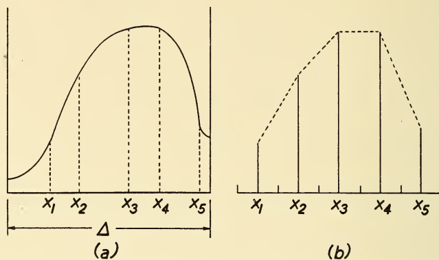
Fig. 4.—(a) A point in \infty -space; (b) its principal projection on the x_1 - x_2 - x_3 - x_4 - x_5 hyperplane.
