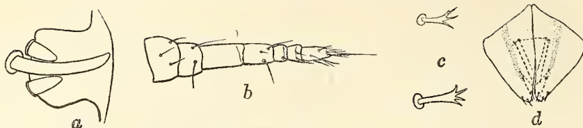
FIG. 33. Coccus viridis (Green), adult female; a, spiracular spines, \times 640 ; b, antenna, \times 165 ; c, marginal spines, \times 640 ; d, anal plates from above, \times 165 .
