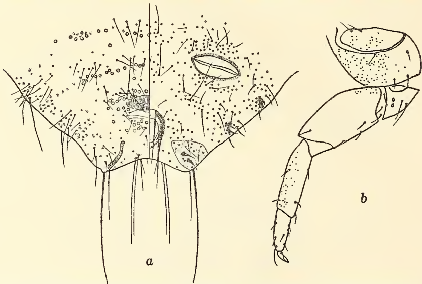
FIG. 18. Pseudococcus lilacinus Ckll., adult female; a , posterior apex of abdomen, showing cerarii, ventral chitinized thickening, anal ring, apical setæ, etc., \times 115 ; b , hind leg, showing numerous minute pores on coxa and tibia, \times 115 .
