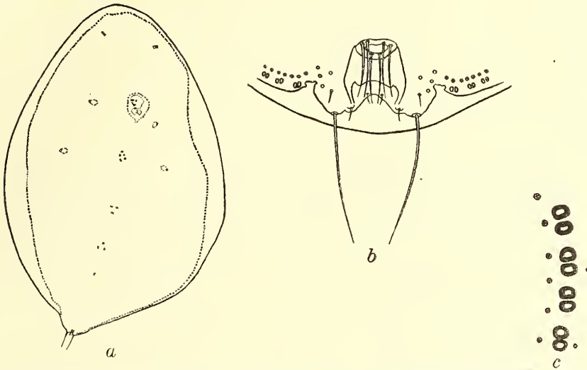
FIG. 8. Asterolecanium bambusæ (Edv.), adult female; a, outline of body, showing marginal pores, dorsal pores, antennæ, spiracles, mouth parts, \times 32 ; b, caudal apex of body, showing anal ring and lobes, \times 325 ; c, detail of marginal double-pore band, \times 640 .
