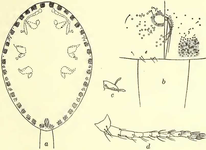
FIG. 10. Puto spinosus (Rob.), adult female; a , outline of body, showing principally the chitinized gland- and spine-bearing areas along the body margin, \times 38 ; b , apex of abdomen, showing posterior chitinized area, anal and genital openings, and apical seta, \times 110 ; c , claw, showing denticle, \times 325 ; d , antenna, \times 115 .
