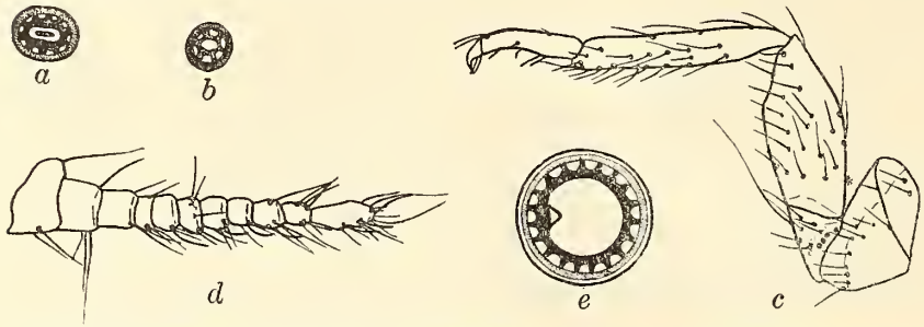
FIG. 3. Icerya seychellarum (Westw.), adult female; a and b, different sorts of solid-center gland pores on body, \times 640 ; c, leg, \times 57.5 ; d, antenna, \times 57.5 ; e, large open-center gland pore, secreting glassy threads, \times 640 .
