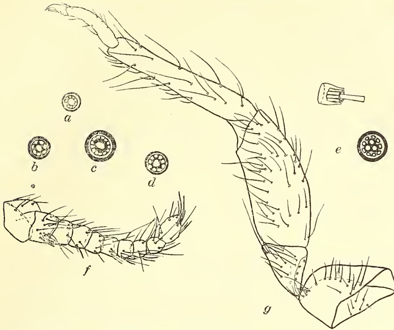
FIG. 1. Icerya jacobsoni Green, adult female; a to d, surface views of various sorts of circular wax gland pores found on body, \times 640 ; e, surface view and section of trilocular center pores found in clusters along body margin, \times 640 ; f, antenna, \times 57.5 ; g, leg, \times 57.5 .
