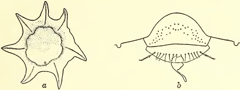
FIG. 27. Vinsonia stellifera (Westw.), adult female; a , outline of body, showing pointed secretory projections, \times 12 ; b , anterior portion of body, showing suture separating off the "head" and the antennæ, \times 57.5 .
