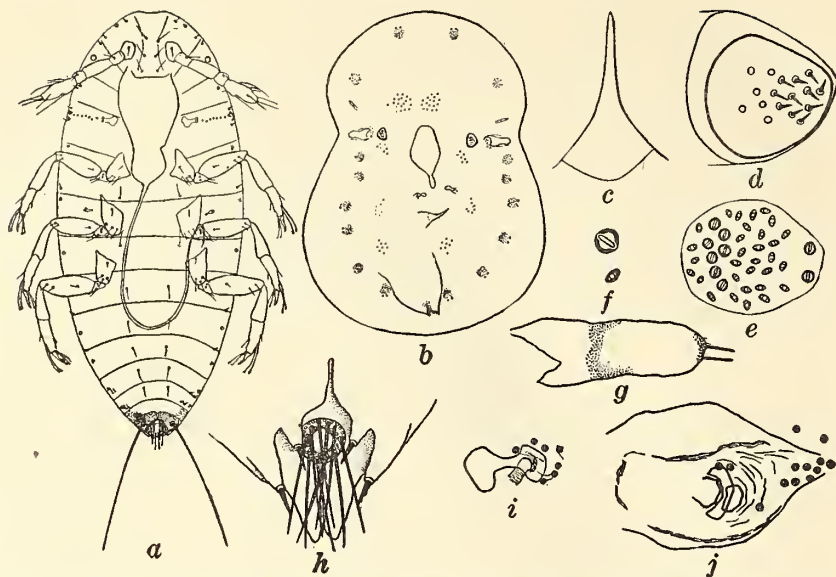
FIG. 21. Tachardia minuta sp. nov., young larva; a , from beneath, \times 165 ; adult female, b , outline of body, showing position of various organs, \times 38.5 ; c , dorsal spine, \times 230 ; d , stigmatic plate, \times 335 ; e , marginal group of gland pores, \times 335 ; f , details of pores in same, \times 640 ; g , antenna, \times 335 ; h , apex of anal lobe, \times 335 ; i and j , spiracles, \times 335 .
