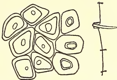
FIG. 38. Saissetia nigra (Nietn.), adult female, showing derm areolation, marginal and spiracular spines, \times 165 .
