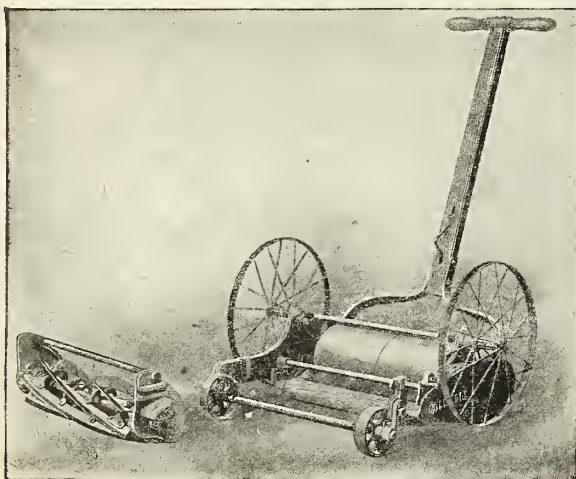
Coldwell's Demountable Putting-Green Mower
