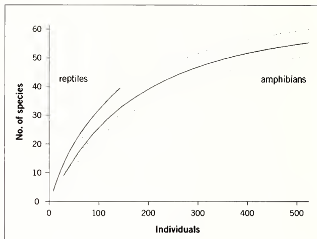
Figure 21. Species accumulation curves for amphibians and reptiles recorded over 18 days at the four rapid inventory campsites in Peru's Kampankis Mountains.
