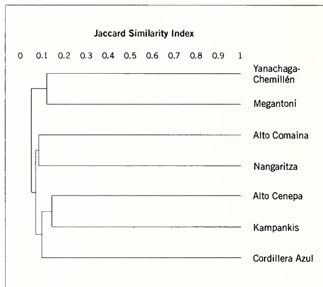
Figure 20. Cluster analysis comparing the fish species composition of Peru's Kampankis Mountains with that of six other mountainous areas in Peru and Ecuador.
