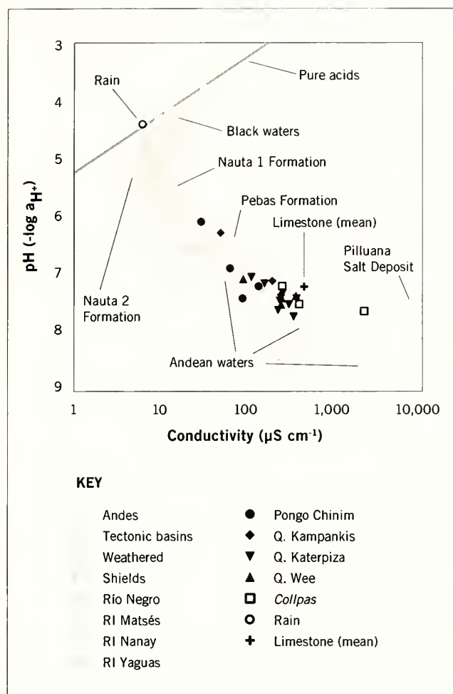
Figure 18. Field measurements of pH and conductivity (in micro-Siemens per cm) of various South American water bodies. The solid black symbols represent streamwater samples collected during this study. The solid light gray symbols represent samples collected during three previous inventories: Matsés (RI16), Nanay-Mazán-Arabela (RI18), and Yaguas-Cotuhé (RI23). The open light gray symbols correspond to numerous samples collected elsewhere across the Amazon and Orinoco basins. Note that streams from each site tend to group together and that we can characterize these groupings according to their geology and soils. In the Amazon lowlands of eastern Peru, four groups stand out: the acid black waters associated with quartz-sand soils, the low-conductivity waters associated with the Nauta 2 sedimentary unit, the slightly more conductive waters of the Nauta 1 sedimentary unit, and the substantially more conductive and higher-pH waters that drain the Pebas Formation. The most dilute waters are simply rain with tiny quantities of added cations (Nauta 2) or organic acids (black waters). Typical Andean waters overlap with the Pebas Formation, but extend to considerably higher conductivities and pH. The waters of the Kampankis Mountains span the range from Pebas-like waters to waters that drain limestones (+ symbol). Three collpa (salt-lick) samples are indicated. The two with lower conductivities are from the Amazon lowlands and are associated with the Pebas Formation. Their compositions can be explained from the dissolution of calcite and gypsum, two minerals found in the Pebas Formation. The high-conductivity collpa from near the Quebrada Wee campsite can only be explained by the dissolution of rock salt. Rock salt is not exposed at the surface in the Kampankis Mountains, but the salt itself or waters affected by the salt appear to come up to the surface along faults. The Quebrada Wee collpa is located on one such fault. The salty formation in the Kampankis subsurface is exposed at the surface in the Pilluana salt deposit near Tarapoto, Peru.
