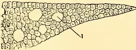
Vertical section of half a leaf of a Potamogeton, with air-spaces I.
