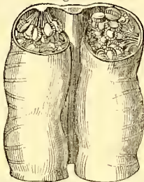
Struthiopteris germanica. Portion of a pinna with the rolled margins covering the sori. Magnified 40 diameters.
