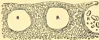
Section of the rind of an orange, showing the internal glands, R, R. Magn. 50 diams.
