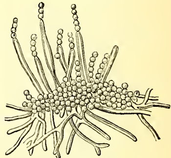
Torula sacchari (aërial form). Magnified 200 diameters.
