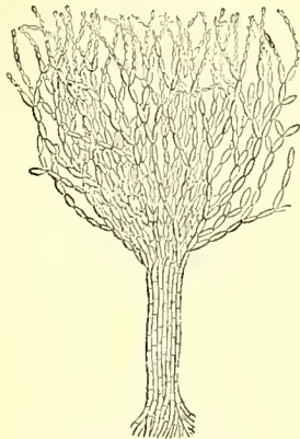
Coremium niveum , Corda. Magnified 200 diameters.
