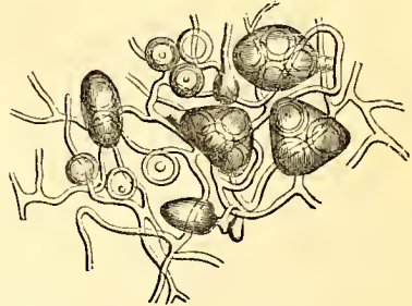
Fig. 184. Elaphomyces hirtus . Section, nat. size.
