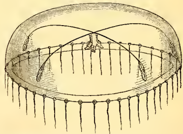
Thaumantias hemispherica , magnified 2 diameters.
