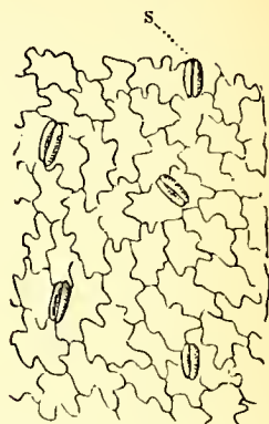
Epidermis from petal of the balsam, with stomata, S. The ep dermal cells here have elegantly sinuous side-walls. Magnified 200 diameters.
