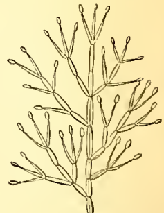
Fig. 344. Cephalothecium roseum . Magn. 200 diams.
