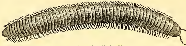
Iulus terrestris . Magnified 4 diameters.
