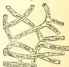
Mougeotia genulifera . Conjugating filaments. Magnified 100 diameters.
