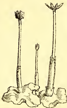
Anicura pinguis. Bursting sporanges. Magnified 2 diameters.
