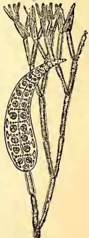
Dasya Kützingiana . Magnified 50 diams.
