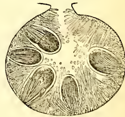
Section of a conceptacle of F. canaliculatus , containing sporangies, antheridia, and paraphyses.
