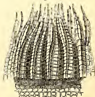
Bryum intermedium . A portion of the peristome. Magnified 150 diameters.
