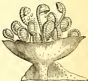
Deparia prolifera. Sorus enclosed in the stalked indusium. Magnified 25 diameters.
