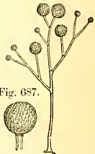
Fig. 685. Mystrosporium Stemphylium , Corda ( Stemphylium , Fries). Magn. 200 diams.
