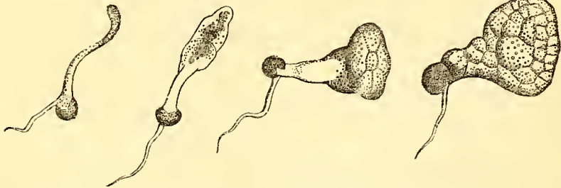
Germination of Pteris longifolia . Magn. 100 diams.
