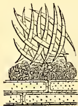
Fig. 688. Leptotrichum glaucum . Free spores among the filaments of the matrix. Magn. 200 diams.
