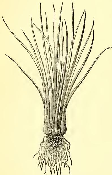
Isoëtes setacea. Natural size.
