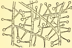
Acremonium fuscum (magnified).
