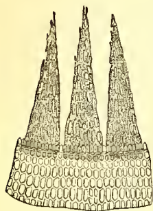
Fig. 476. Coscinodon pulvinatus . Fragment of peristome. Magn. 100 diams.
