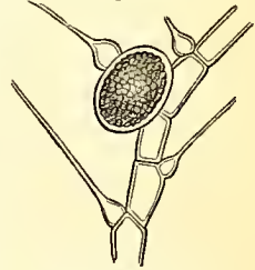
Bulbochæte setigera. Portion of a filament with a sporicell. Magnified 150 diameters.
