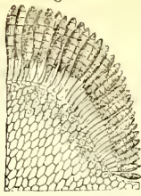
Coryneum disciforme. Vertical section of half a pustule. Magnified 200 diams.
