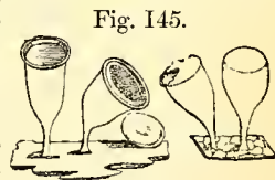
Craterium pyriforme. Magnified 10 diameters.
