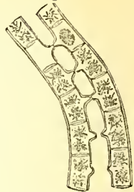
Zygnema cruciata . Conjugating filaments. Magnified 250 diameters.
