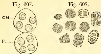
Fig. 607. Parent cells of pollen-grains just after the separation of the contents into four portions, treated with iodine. C M , the parent cell. P , the protoplasmic portions, each with a nucleus and a well-defined outline at the surface of the primordial utricle. Magnified 250 diameters.
