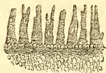
Pottia cæspitosa . Fragment of peristome. Magnified 50 diameters.
