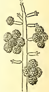
Botryosporium pulchrum. A fertile filament bearing sporiferous lateral branches.
