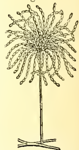
Briarea penicillata . Magnified 200 diameters.
