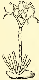
Botrytis. Magnified 200 diameters.
