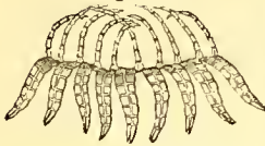
Fig. 481. Raconitrium fasciculare . Section of margin of sporange, with a tooth of the peristome. Magn. 100 diams.
