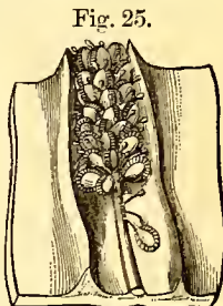
Antrophyum Lessoni. Part of a sorus. Magnified.
