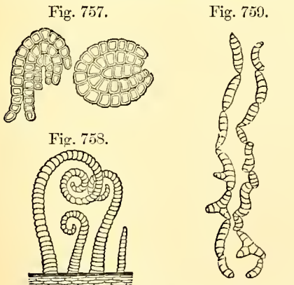
Fig. 757. Speira toruloides . Magnified 200 diameters. Fig. 758. Gyrocercus ammonis . Magnified 200 diams. Fig. 759. Trimmatostroma salicis . Magn. 200 diams.
