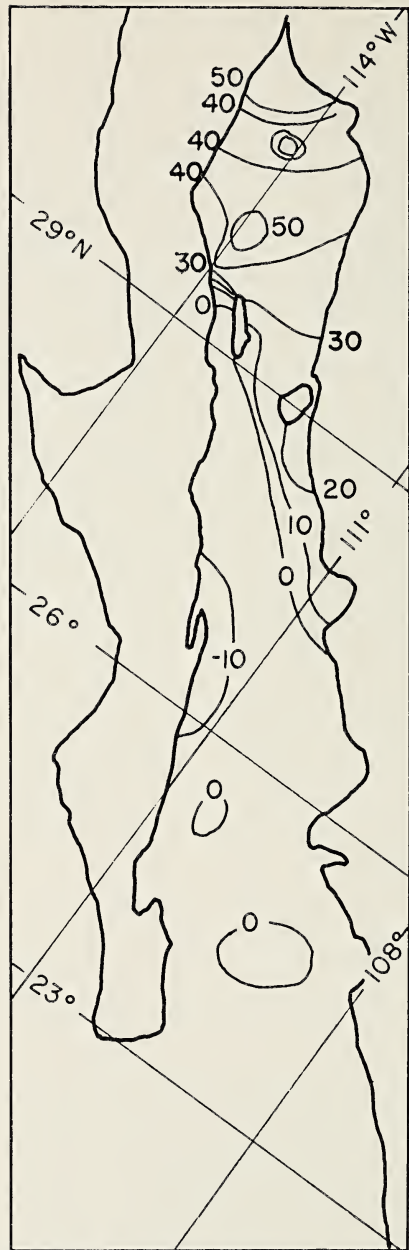
OXYGEN SUPERSATURATION (‰)
