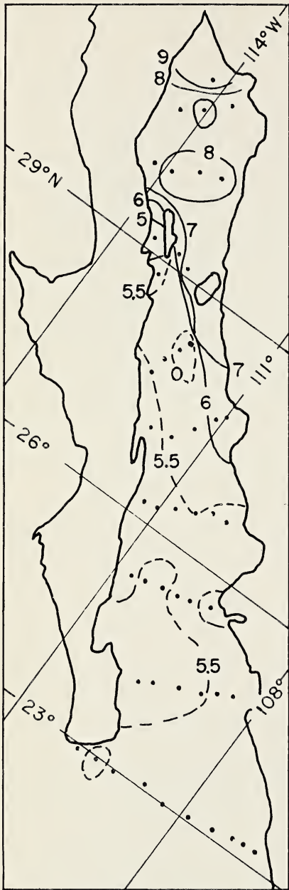
OXYGEN (ml/L)
