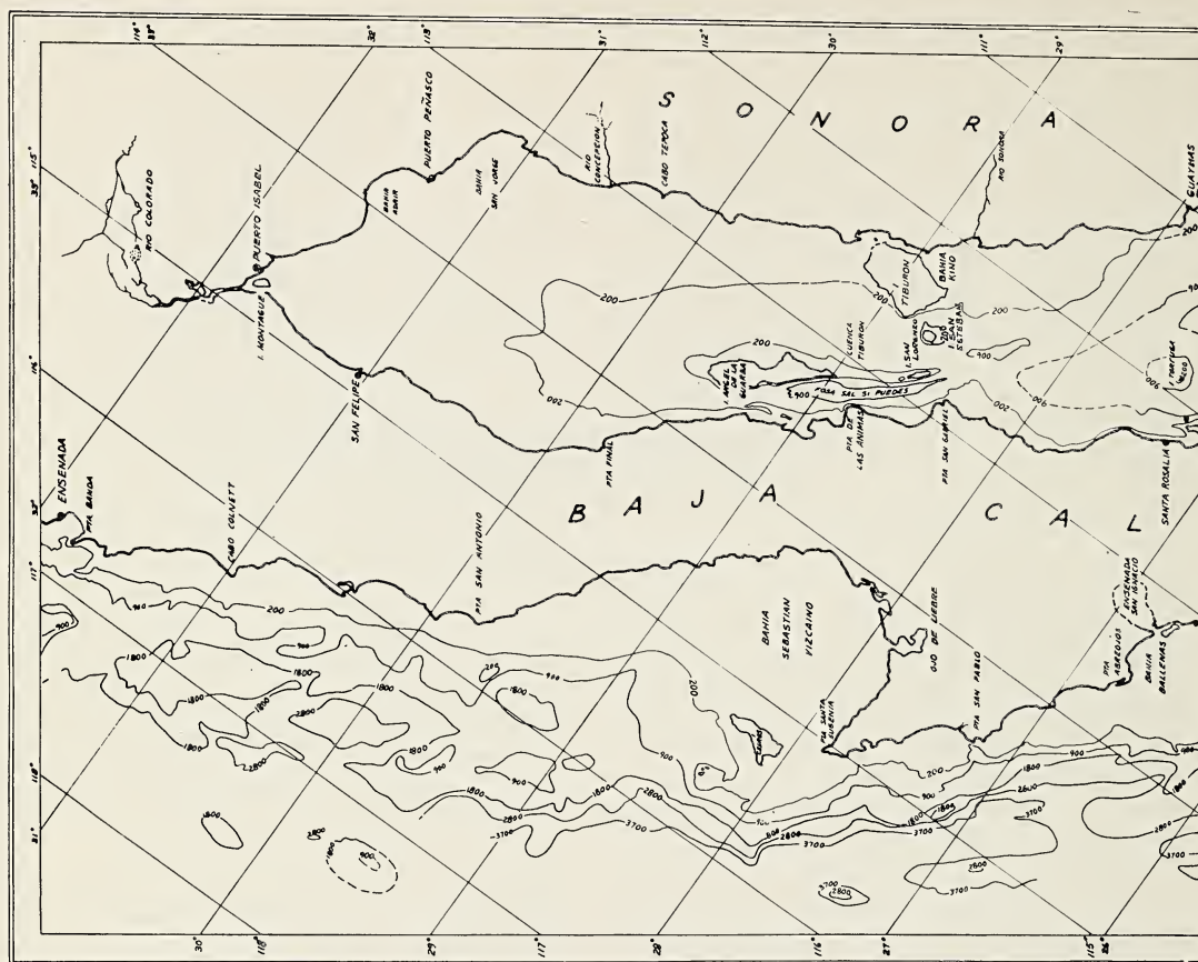
FIG. 1. Bathymetric map of the Gulf of California.
