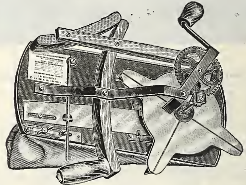
The Rittenhouse Seeder, No. 3
