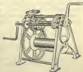
Crab (c).
