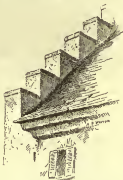
Corbel-steps.—Castle of Schaffhausen, Switzerland.
