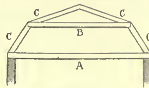
Diagram of Curb-roof. A, tie-beam; B, collar-beam; C, rafters.
