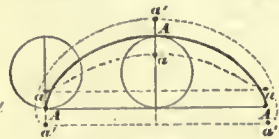
Cycloids.
