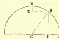
Cosine.
