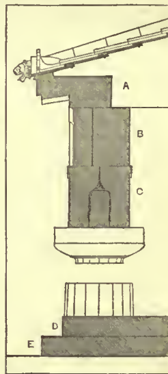
Doric Cornice Construction, Assos. (From Papers of the Archaeol. Inst. of America, I, 1882.)
