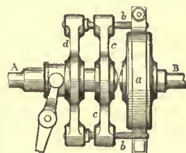
Slip-clutch Coupling.
