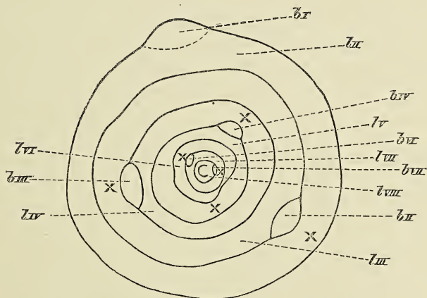
Fig. 2. Transverse section through a bud of Calamus sp. showing seven leaves ( l_{ii} — l_{viii} ): the midrib of each is marked thus x: opposite each midrib, excepting those of l_v and l_{viii} , is seen an axillary bud ( b_{ii} — b_{vii} ): the outermost bud ( b_i ) is the axillary bud of the next outer leaf, which has been removed. ( \times 20 .)
