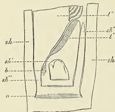
Fig. 3. Longitudinal section through a bud of Calamus sp.; l^I, l^{II} laminae; sh, sh^I, sh^{II} sheaths of corresponding leaves; n node; b bud in the axil of l^{II} , and already adherent to sheath of l^I . ( \times 10 ).
