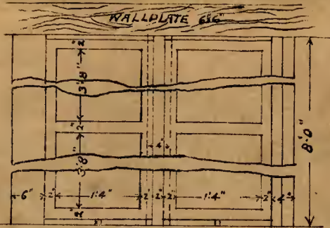
ELEVATION DETAIL 1/2 INCH TO 1 FOOT SCALE
