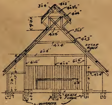
SECTION
