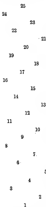
Vertical Projection of the \frac{3}{8} Arrange- ment.
