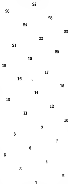
Vertical Projection of the \frac{5}{13} Arrangement.
