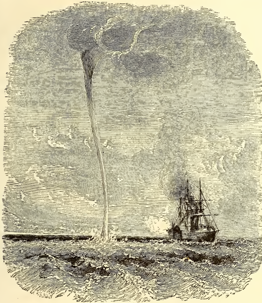
WATERSPOUT.
