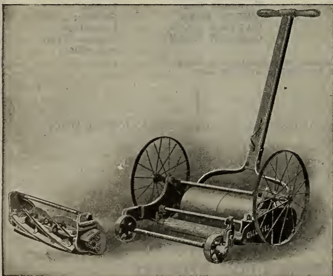
Coldwell's Demountable Putting-Green Mower
