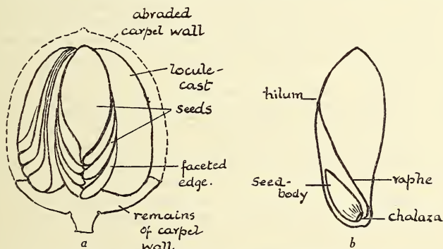
FIG. 5.— Toona sulcata . a, cast of fruit showing the arrangement of the seeds in the locules. Diagrammatic. b, seed (diagrammatic) to show structure.
