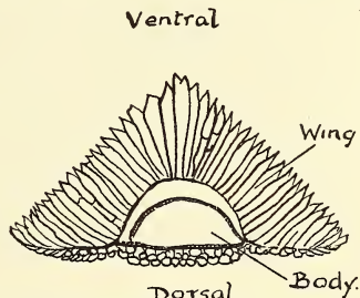
FIG. 16.—Diagrammatic transverse section of seed of Palaeocharidium cellulare .
