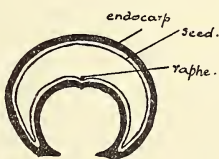
FIG. 4.—Diagrammatic transverse section across an endocarp of Tinospora excavata .
