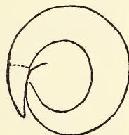
FIG. 12.— Cupanoides grandis Bowerbank. Seed with testa removed (diagrammatic) to show the form of the radicle and (in part) of the cotyledons. The folding of the inner cotyledon is obscure. The broken line indicates a probable transverse constriction or furrow on the radicle.
