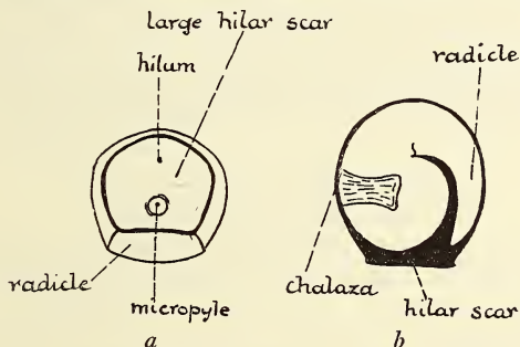
FIG. 10.— Palaealophylus ovoides . a , base of seed showing hilar scar (diagrammatic); b , diagrammatic side view of seed from which the testa has been removed, showing the radicle and chalaza.
