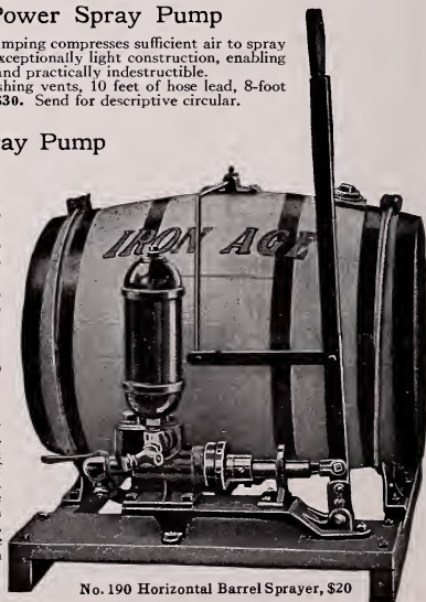
No. 190 Horizontal Barrel Sprayer, $20
