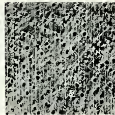
FIG. 78.—Serial patch.
