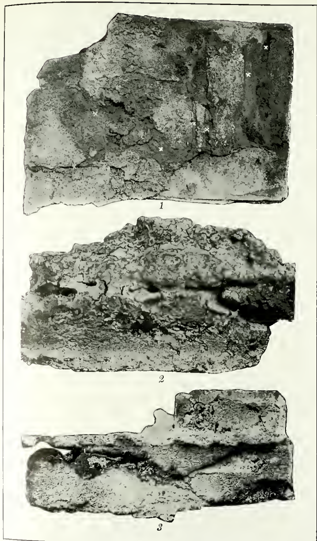
PLATE VII. TERMITES IN BRICK WALLS.
