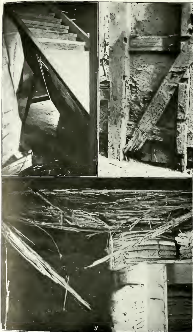
PLATE V. DAMAGE DONE BY TERMITES.
