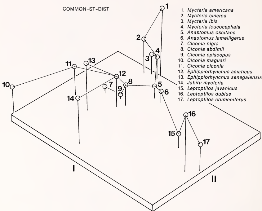
Fig. 14.—Three-dimensional model showing arrangement of storks in phenetic space based on a multidimensional scaling analysis of sternum characters transformed using the COMMON procedure. A minimum spanning network derived from taxonomic distances calculated from the transformed data is superimposed on the model.
