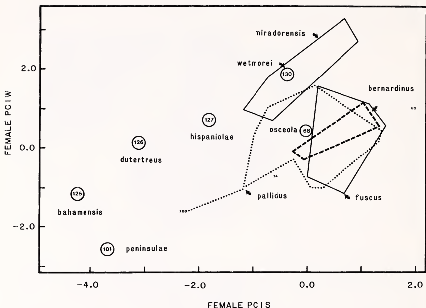
Fig. 7.—Plot of the first principal component of wing variation (PC1W) versus the first principal component of skull variation (PC1S) for 96 geographic groups of female Epptesicus fuscus . Circled GG numbers indicate insular and peninsular subspecies (see Fig. 2). Polygons enclose the GG's for each continental subspecies as defined by Hall (1981). GG's 74 and 89 are outliers from E. f. fuscus .
