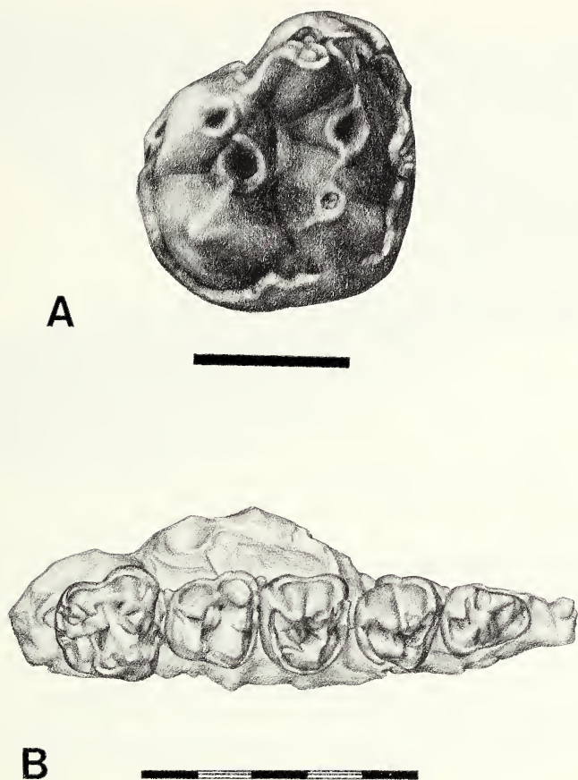
Fig. 4.— Pilgrimella pilgrimi (= Anthracobune pilgrimi ); all scale units equal 1 cm. a) Munich 1956 II 20, holotype; b) LUVP 15006.
