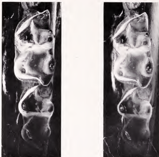
Fig. 1.— Peratherium edwardi , USNM 19200, LM 3-4 , type; approx. \times 14 .
