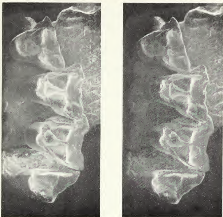
Fig. 3.— Peradectes elegans . (C) AMNH 17369, LM 1-4 , paratype; approx. \times 16.5 .
