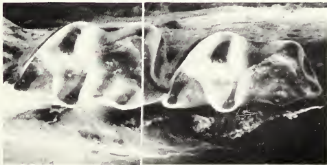
Fig. 2.— Peratherium knighti : (A) YPM 13514, M_4 (type of Entomacodon minutus ); (B) CM 42135, RM_{3-4} (from Tabernacle Butte, the type locality); (C) PU 16115, RM_{2-3} (type of P. morrisi ); all approx. \times 15 .
