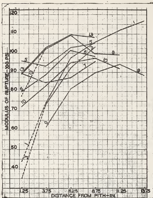
Fig. 2.-Modulus of rupture plotted over distance of the test piece from the pith, for representative bolts of green tabomoo. Dotted lines indicate data from rejected material.
