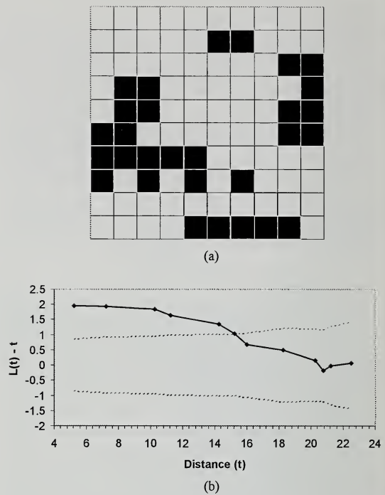
FIG. 2. An example plot showing the distribution of occupied quadrats (a) and the corresponding graph of the K-function (b). The dashed lines represents a 95% confidence interval based on 1000 Monte Carlo simulations. The graph (b) shows significant clumping on the plot up to 15 cm. This value was this plots contribution to the ANOVA for the experiment as a whole.
