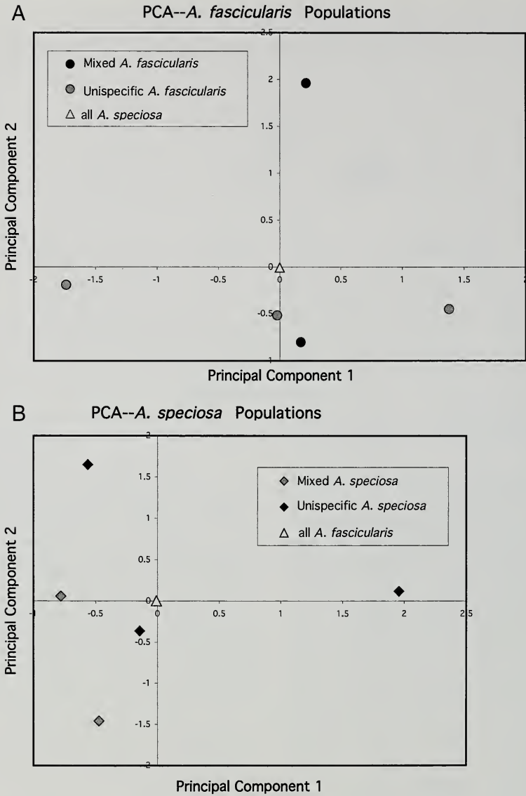
FIG. 7. Two-dimensional scatterplot of first and second principal component scores after PCA based on OTU's for population means of: (A) unispecific and mixed A. fascicularis (Table 1) relative to mean for all A. speciosa populations. (B) unispecific and mixed populations of A. speciosa relative to mean for all A. fascicularis populations.
