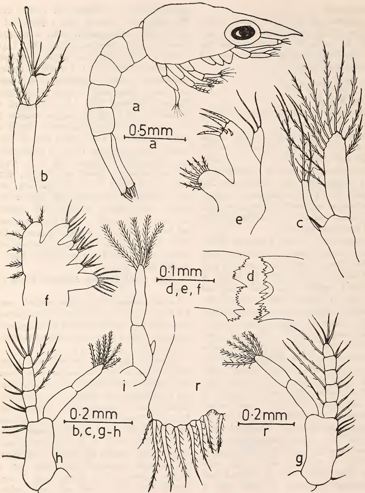
Fig. 2. Second zoea, Clibanarius aequabilis var. merguensis de Man. a, entire larva; b, antennule; c, antenna; d, mandibles; e, first maxilla; f, second maxilla; g, first maxilliped; h, second maxilliped; i, third maxilliped; r, telson.
