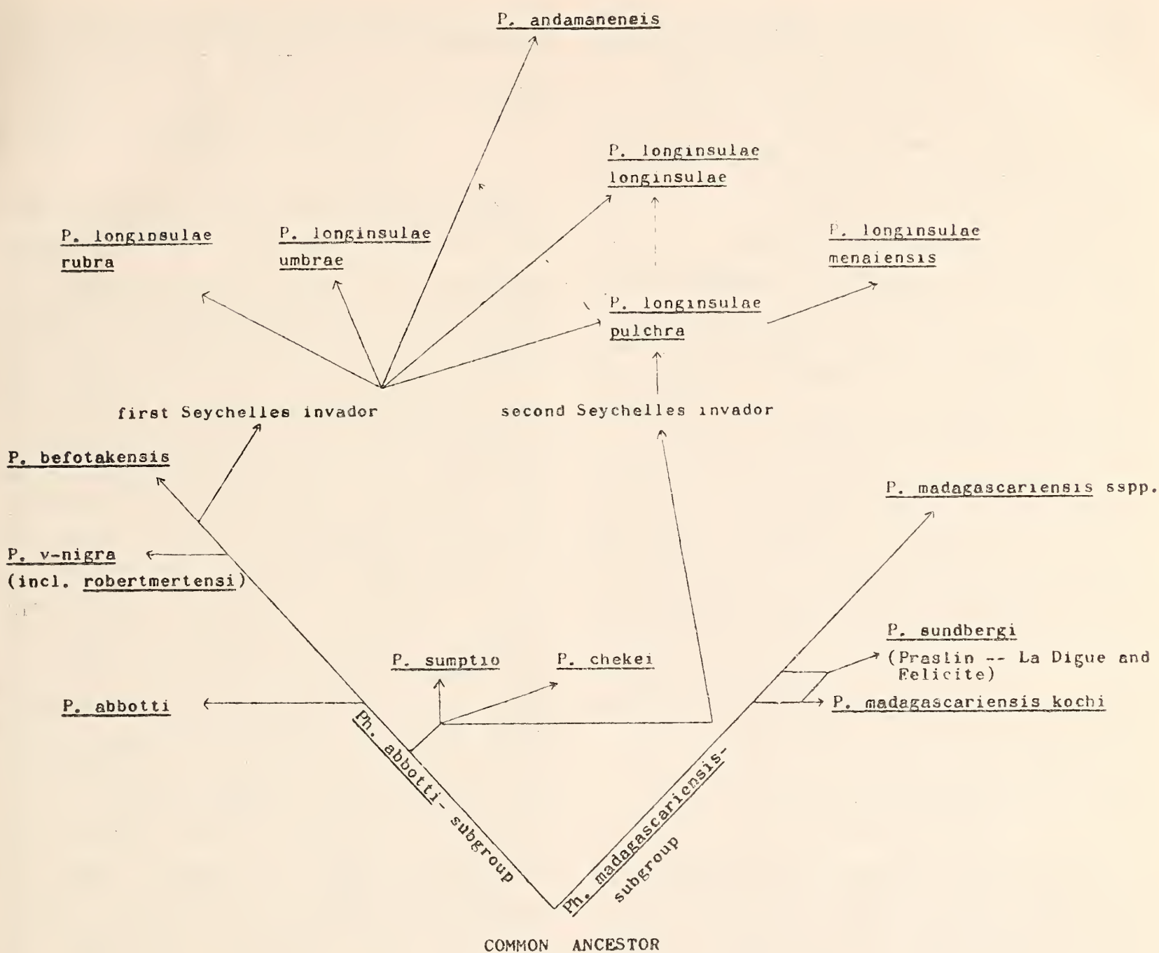
Fig. 2. Phylogenetic tree.
