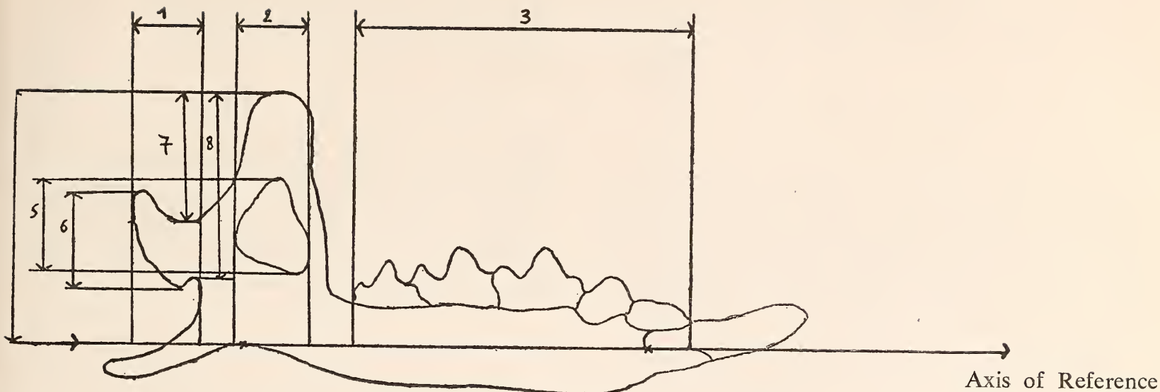
Fig. 1. Mandibular measurements.
