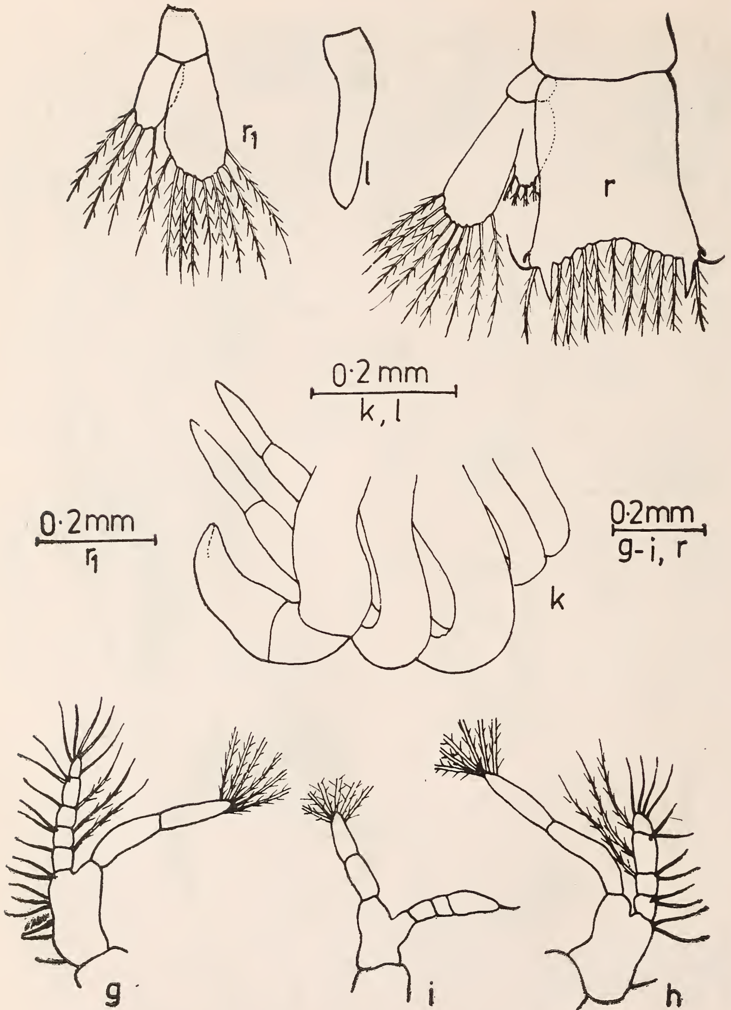
Fig. 5. Fourth zoea, Clibanarius aequabilis var. merguiensis de Man. g, first maxilliped; h, second maxilliped; i, third maxilliped; k, pereiopods; l, pleopod; r, telson and r_1 , uropods.
