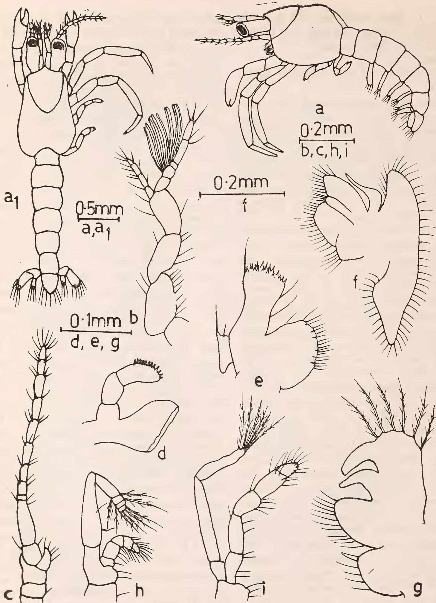
Fig. 6. Glaucothoe of Clibanarius aequabilis var. merguiensis de Man. a, lateral view of entire larva; a 1 , dorsal view of entire larva; b, antennule; c, antenna; d, mandible; e, first maxilla; f, second maxilla; g, first maxilliped; h, second maxi- lliped; i, third maxilliped.
