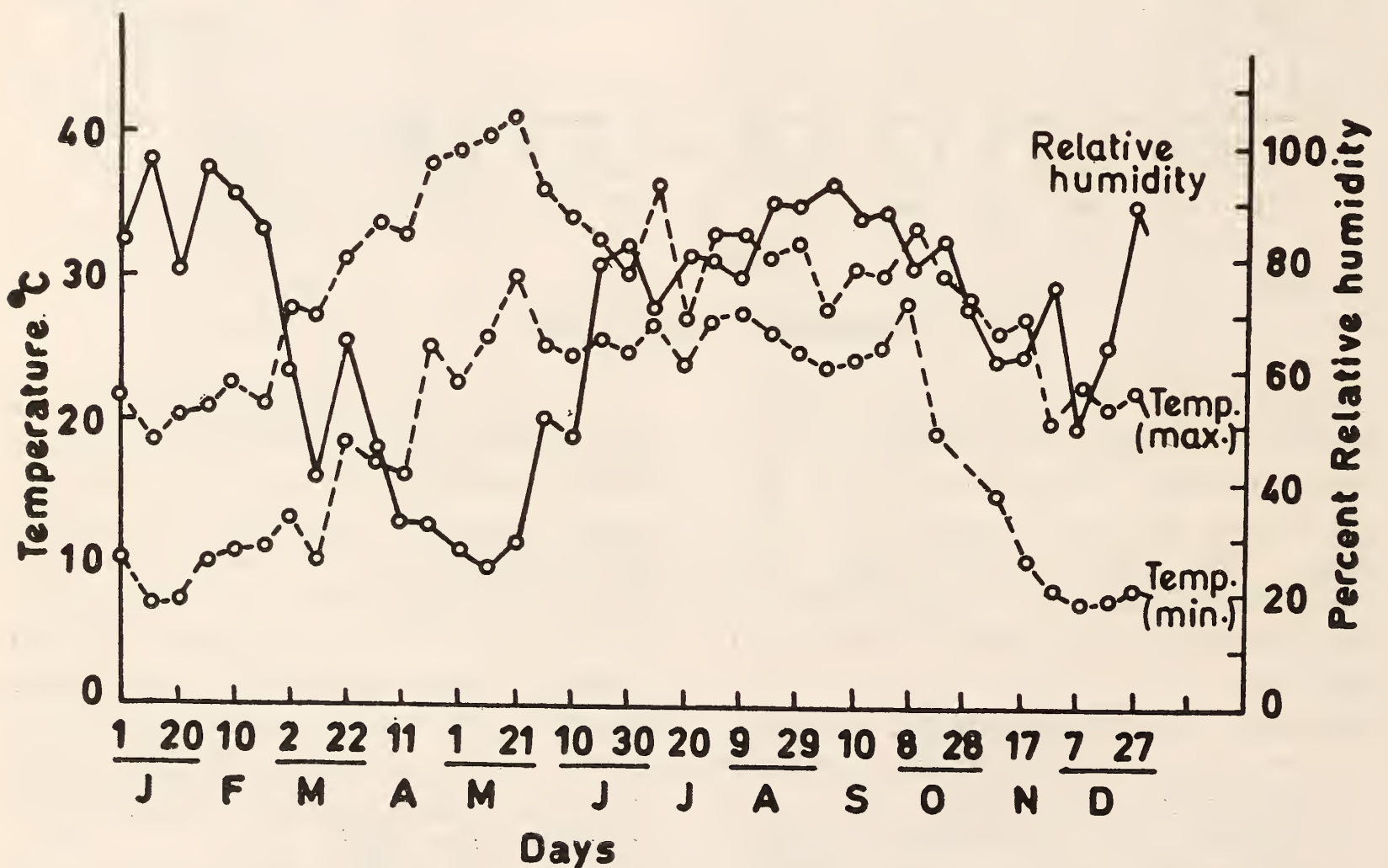
FIG. 2 CLIMATIC DATA 1975
