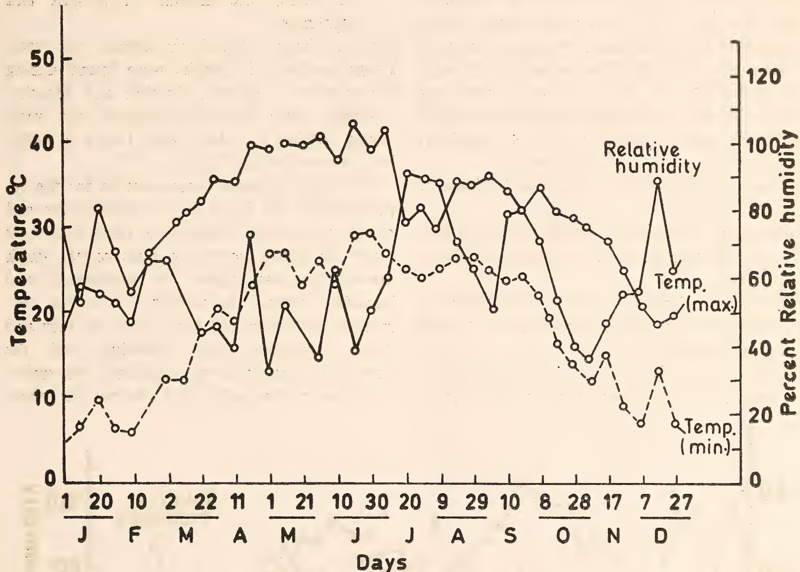
FIG.1 CLIMATIC DATA 1974
