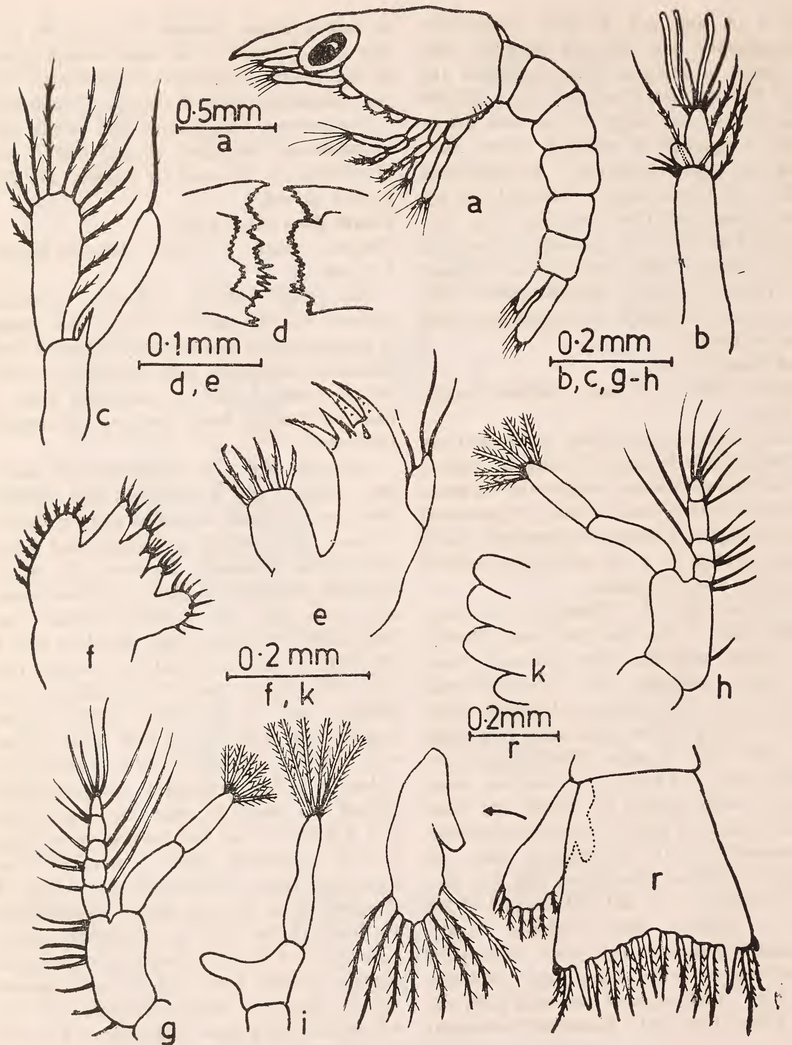
Fig. 3. Third zoea, Clibanarius aequabilis var. merguensis de Man. a, entire larva; b, antennule; c, antenna; d, mandible; e, first maxilla; f, second maxilla; g, first maxilliped; h, second maxilliped; i, third maxilliped; k, pereopods; r, telson.
