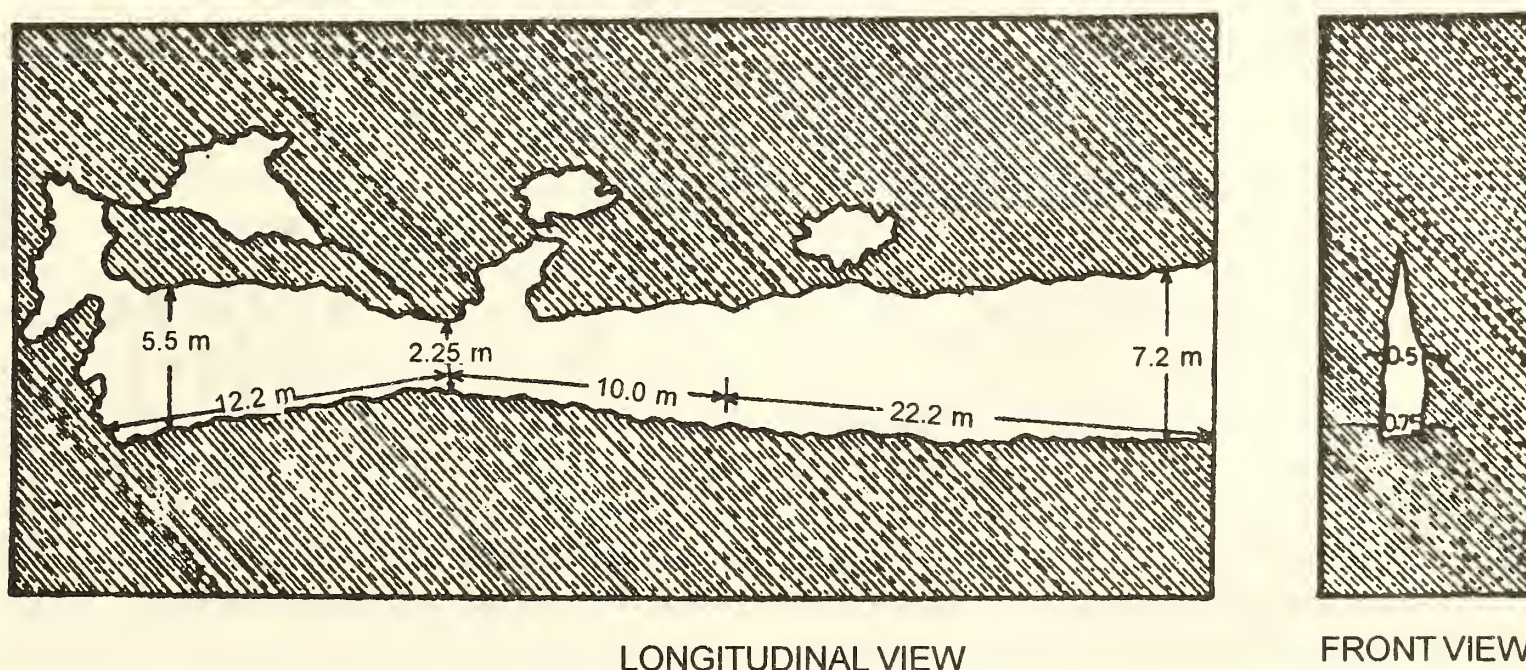
Fig. 9: Topology and dimensions of the cave inhabited by the colony of Rhinopoma hardwickei
