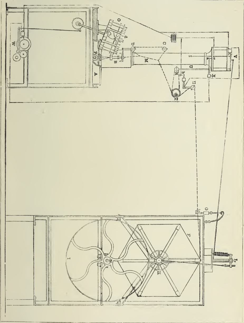
PRINCIPLES OF THE SERRELL AUTOMATIC REEL.
