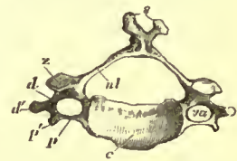
Third Human Cervical Vertebra.
