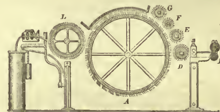
Carding-machine.
