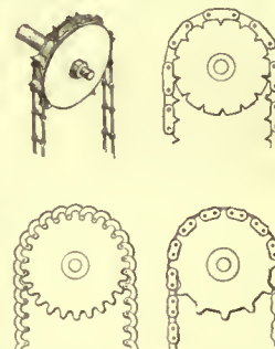
Chain-wheels for transmitting power.
