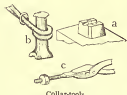
Collar-tools. a, lower half of tool in the hardy-hole of the anvil; b, upper or fuller tool; c, collar and rod in the grip of the pincers.
