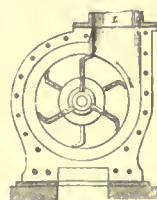
Section of Gwynne's Centrifugal Pump.—The wheel rotates in the direction of the arrow, and delivers the water upward into the induction-pipe, L.
