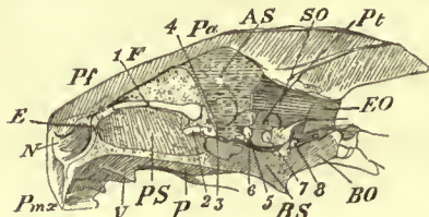
Longitudinal Section of Skull of Turtle ( Chelone mydas ), showing outline of brain in situ, with 1-8, first eight cranial nerves, and the following bones: BO , basioccipital; EO , exoccipital; SO , supraoccipital; BS , basiphenoid; PS , presphenoid; AS , alisphenoid; Pt , pterygoid; Pa , enormously expansive parietal; F , frontal; PF , prefrontal; E , ethmoid; N , nasal; Pmx , premaxilla; V , vomer; P , palatine.
