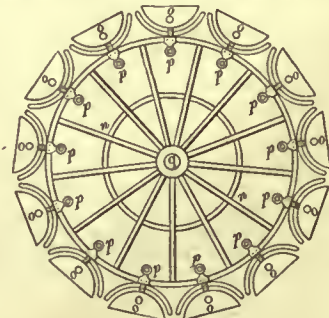
Catoptric Light.
