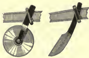
Rolling Colter. Knife-Colter.
