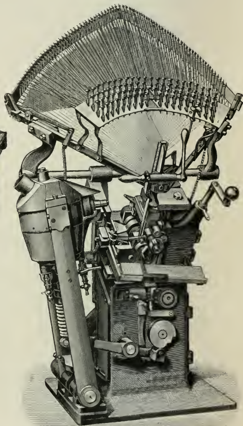
Fig. 3. Typograph.
