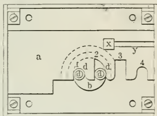
4. Bramah-Schloß.
