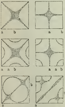
Fig. 15. Chladni's Klangfiguren.
