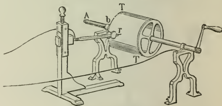
Fig. 21. Phonautograph.
