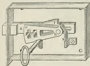
Fig. 8-10. Chubb-Schloß.
