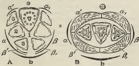
Floral diagrams of Castanea vulgaris , after Eichler. A, diagram of ♂ cyme in axil of catkin-leaf, the sta. and rudimentary gynœceum only shown in the first flr. The sequence of the flrs. is indicated by the figures 1, 2, 3. B, diagram of ♀ partial infl. \delta =bract, \alpha\beta =bracteoles, \alpha'\beta' \alpha , \beta =bracteoles of second order.
