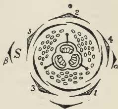
Floral diagram of Hypericum ; after Eichler, ovary cut at base. S the "Schraubel" branch (p. 65).
