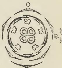
Floral diagram of Anchusa ; after Eichler.
