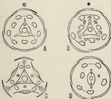
Floral diagrams (after Eichler). A , Rheum ; B , Polygonum tataricum ; C , Rumex ; D , Polygonum lapathifolium . Bracts and bracteoles are omitted, and in C and D the axis also. Glands in B shaded. The asterisks represent missing sta.
