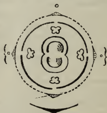
Floral diagram of Asperula , after Eichler.
