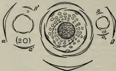
Ranunculus acris . Floral diagram of axillary dichasial cyme, with details of primary flr. Sta. according to the \frac{8}{1} phyllotaxy. \alpha \beta bracteoles of primary, \alpha' \beta' , \alpha , \beta , of later, flrs. After Eichler.
