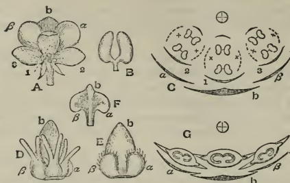
B. alba . A , bract, bracteoles, and perianth, of ♂, from within, with sta. removed; B , a stamen; C , floral diagram of A ; D , bract, bracteoles and flrs. of ♀ from within; E , the same with flrs. removed; F , the same at ripeness of seed; G , floral diagram of D . b =bract; a , β =bracteoles of flr. 1, or bracts of flrs. 2, 3. After Eichler.
