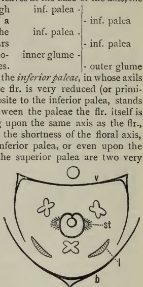
Floral diagram of a grass (after Eichler). b, inferior palea; v, superior palea; l, lodicule; st., stigma.
