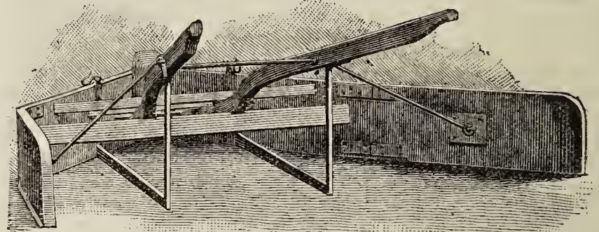
FIG. 28.—THE KNOWSLEY SNOW PLOUGH.
