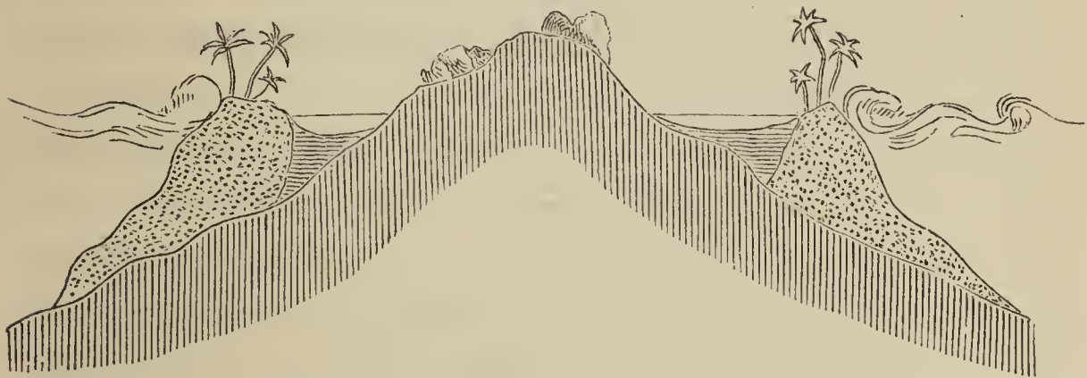
Partially Sunken Island, with an Annular Coral-reef.
