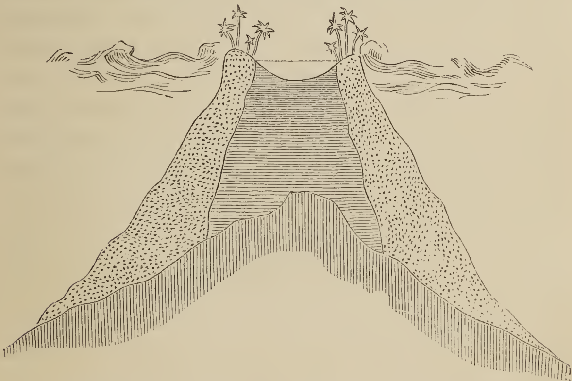
Atoll, or Lagoon-island, as a Coral-structure above a completely Sunken Island.
